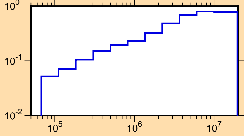
\mu vs. E for ^{44}\text{Ca}(\text{mt251})
