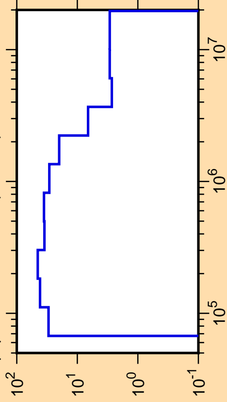
\Delta\mu/\mu vs. E for ^{44}\text{Ca}(\text{mt251})
