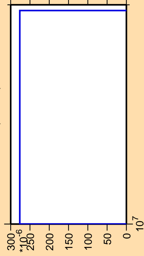
\Delta\sigma/\sigma vs. E for ^{44}\text{Ca}(n,2n\alpha)
