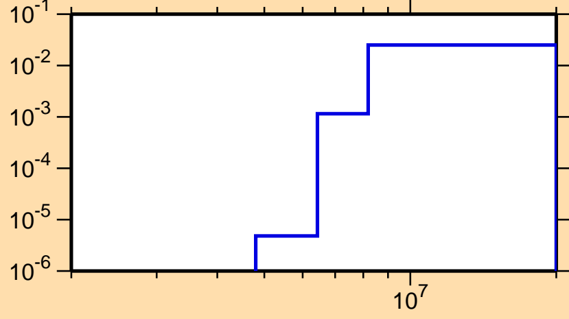
\sigma vs. E for ^{44}\text{Ca}(n,p)
