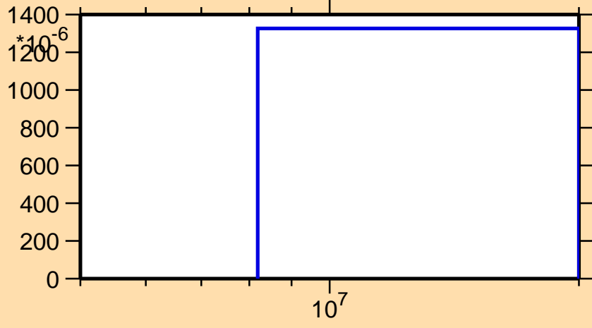
\sigma vs. E for ^{44}\text{Ca}(n,\alpha)
