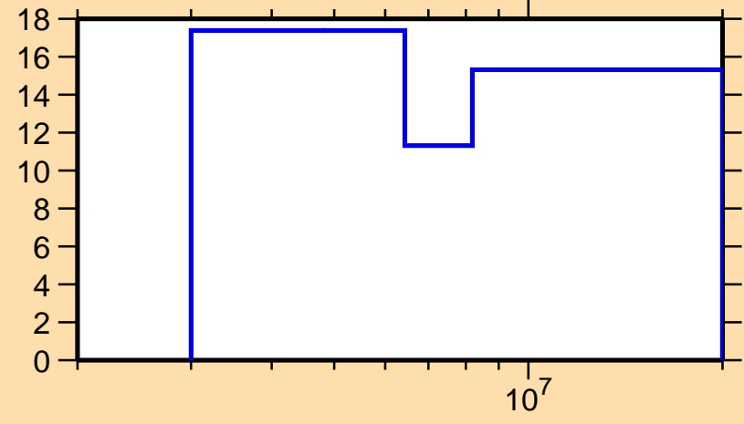
\Delta\sigma/\sigma vs. E for ^{44}\text{Ca}(n,n\text{cont.})
