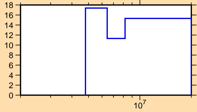
\Delta\sigma/\sigma vs. E for ^{44}\text{Ca}(n,ncont.)
