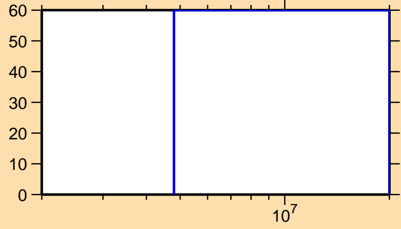
\Delta\sigma/\sigma vs. E for ^{44}\text{Ca}(n,\gamma)
