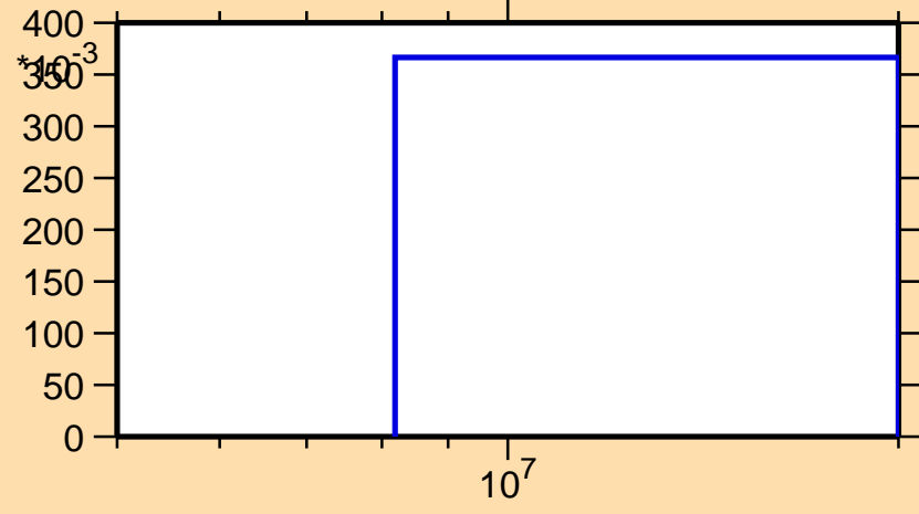
\sigma vs. E for ^{44}\text{Ca}(n,2n)
