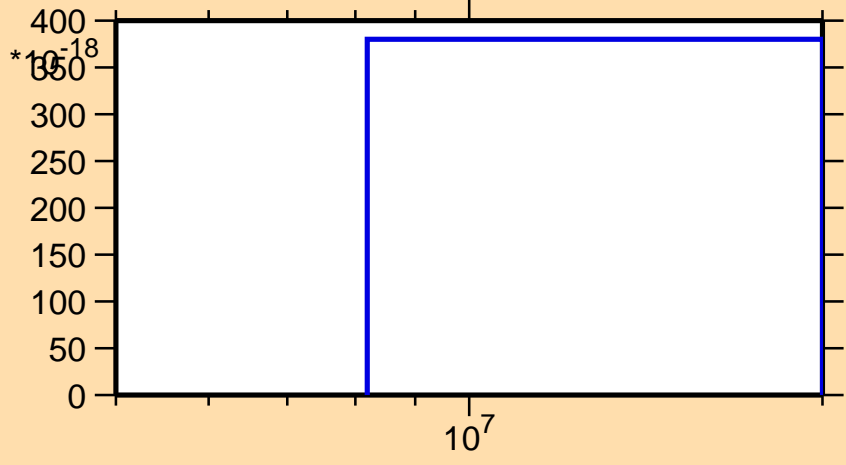
\sigma vs. E for ^{44}\text{Ca}(n,2n\alpha)
