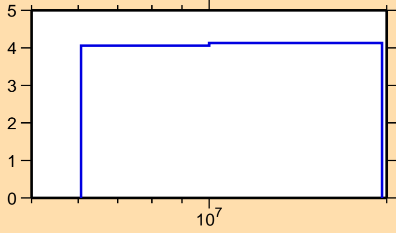
\Delta\sigma/\sigma vs. E for ^{49}\text{Ca}(n,n\text{onel.})
