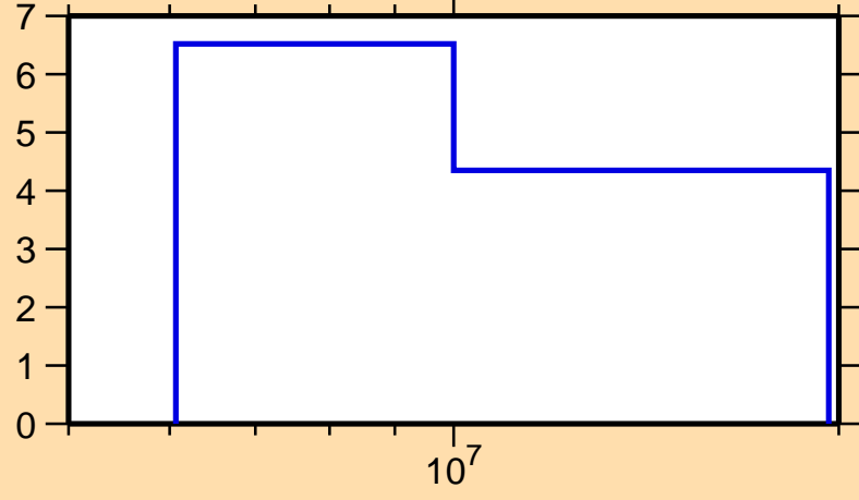
\Delta\sigma/\sigma vs. E for ^{49}\text{Ca}(n,2n)
