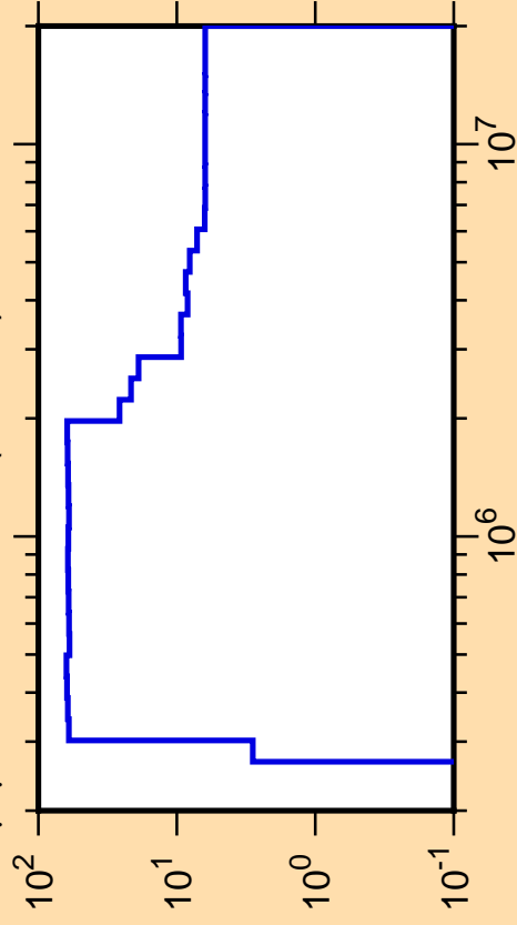
\Delta\mu/\mu vs. E for ^{51}\text{Ca}(\text{mt251})
