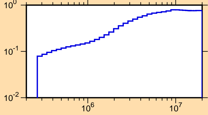
\mu vs. E for ^{51}\text{Ca}(\text{mt251})
