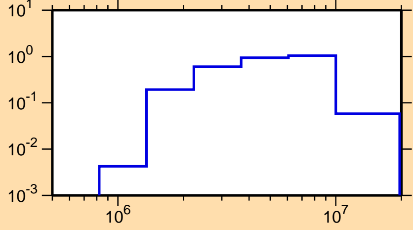
\sigma vs. E for ^{51}\text{Ca}(n,\text{inel.})
