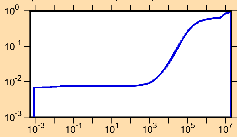
\mu vs. E for ^{97}\text{Cd}(\text{mt251})
