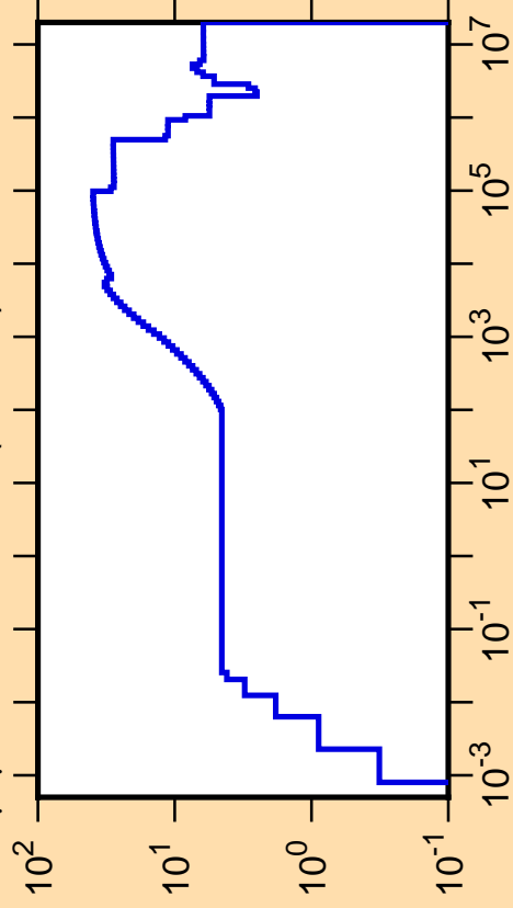
\Delta\mu/\mu vs. E for ^{97}\text{Cd}(\text{mt251})
