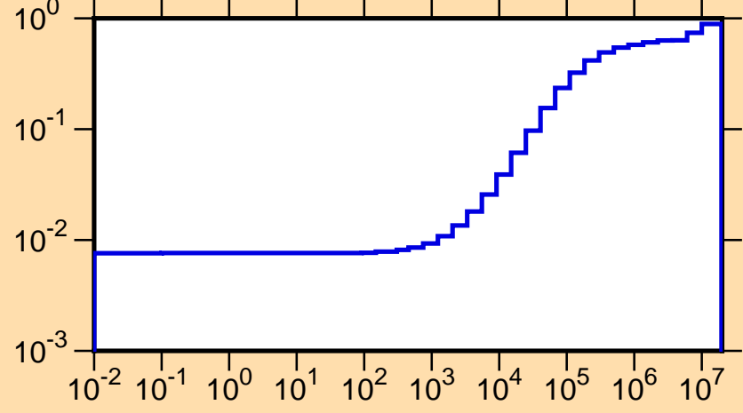
\mu vs. E for ^{97}\text{Cd}(\text{mt251})
