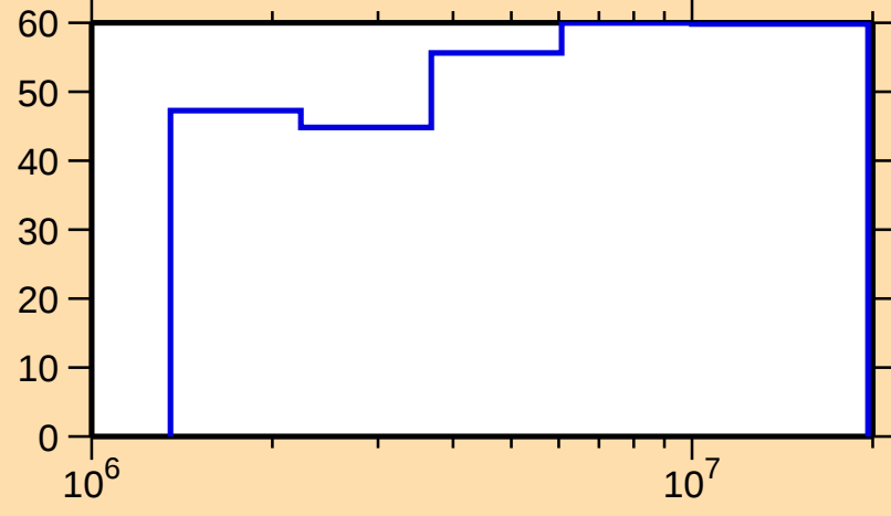
\Delta\sigma/\sigma vs. E for ^{100}\text{Cd}(\text{n},\text{inel.})
