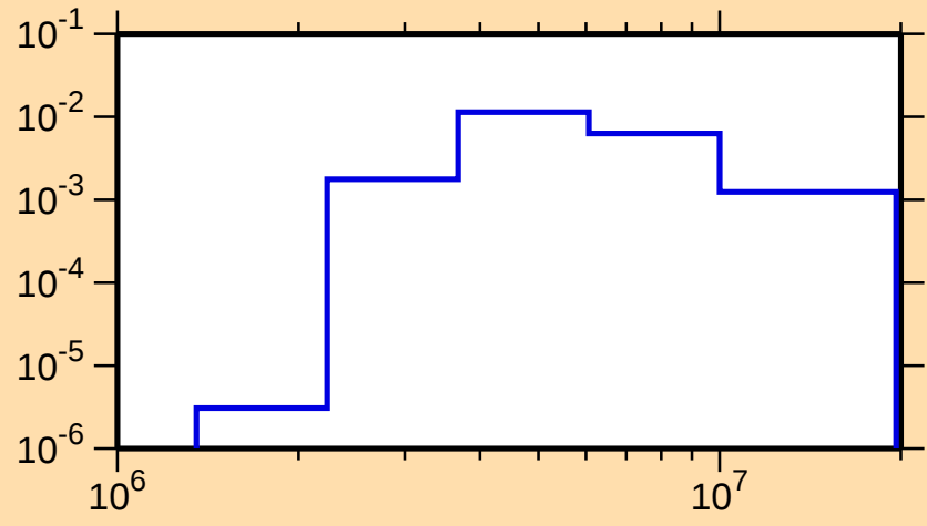
\sigma vs. E for ^{100}\text{Cd}(n,n\text{cont.})
