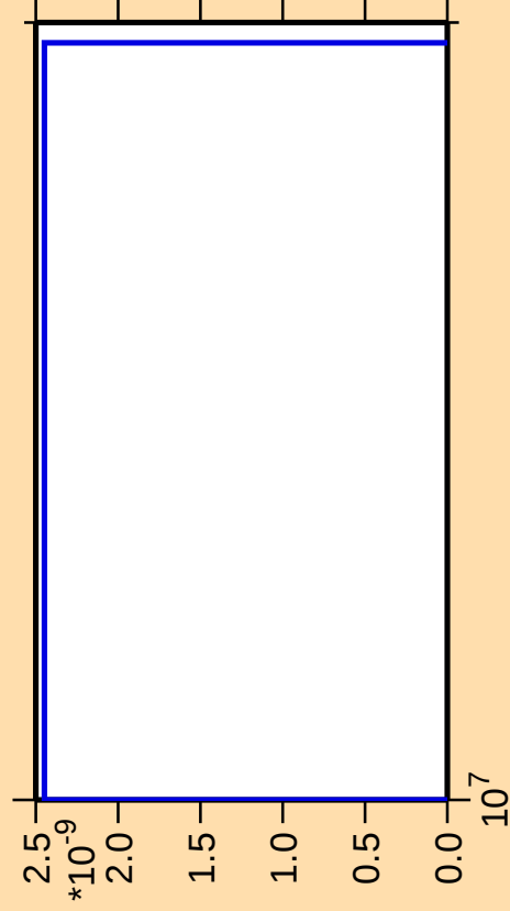
\Delta\sigma/\sigma vs. E for ^{100}\text{Cd}(n,\text{nt})
