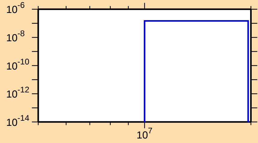
\sigma vs. E for ^{100}\text{Cd}(\text{mt } 45)
