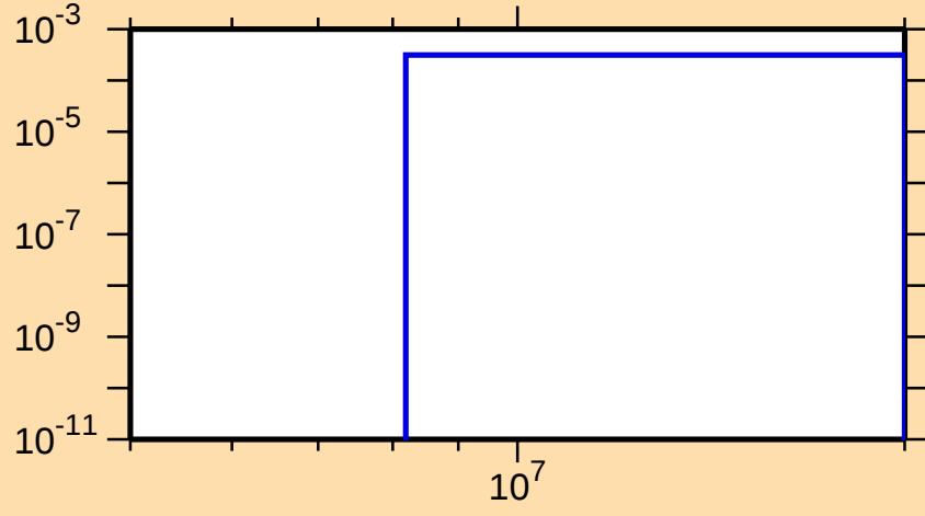
\sigma vs. E for ^{100}\text{Cd}(n,\text{pd})
