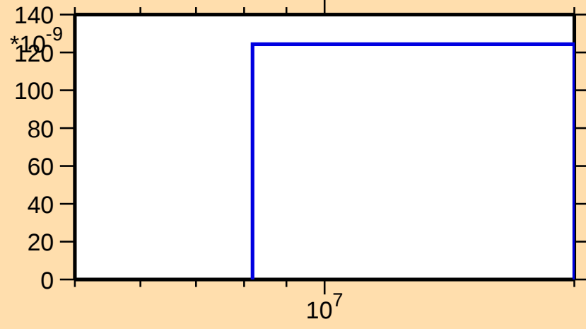
\sigma vs. E for ^{100}\text{Cd}(\text{mt } 45)
