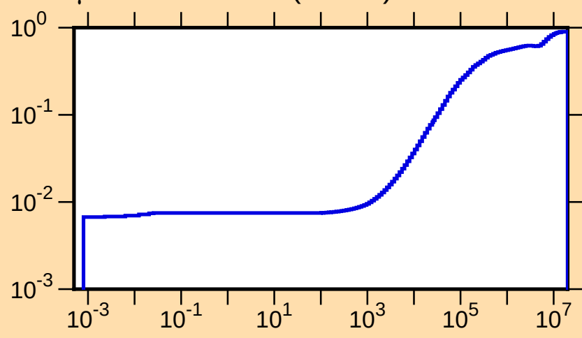
\mu vs. E for ^{101}\text{Cd}(\text{mt251})
