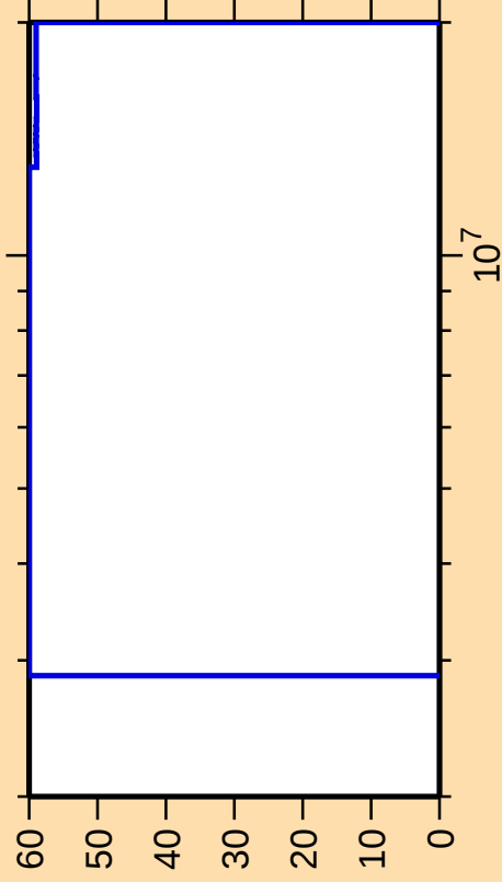
\Delta\sigma/\sigma vs. E for ^{101}\text{Cd}(\text{n,ncont.})
