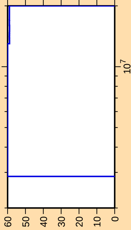
\Delta\sigma/\sigma vs. E for ^{101}\text{Cd}(n,\text{ncont.})
