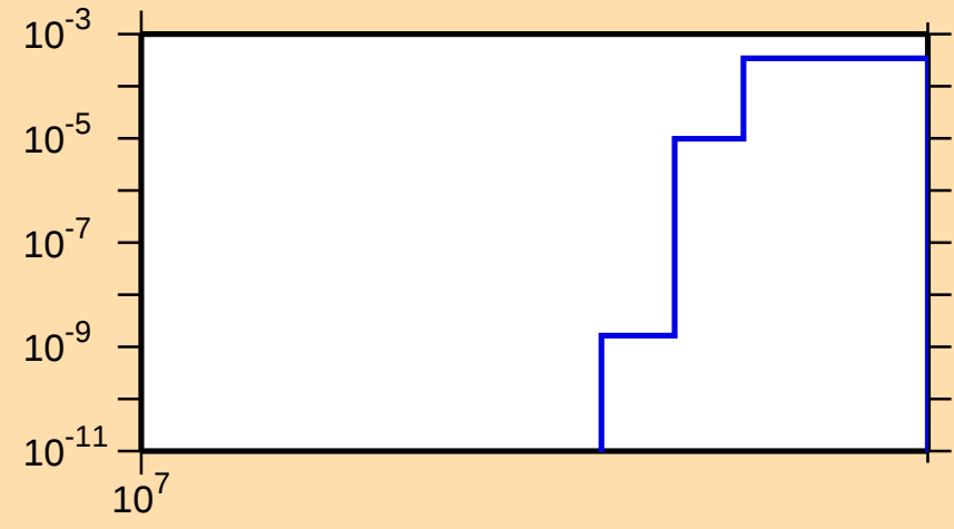
\sigma vs. E for ^{101}\text{Cd}(n,2np)
