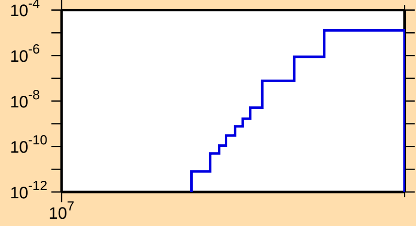
\sigma vs. E for ^{101}\text{Cd}(\text{mt } 45)
