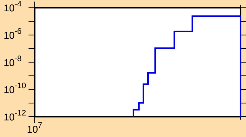
\sigma vs. E for ^{101}\text{Cd}(n,\text{nd})
