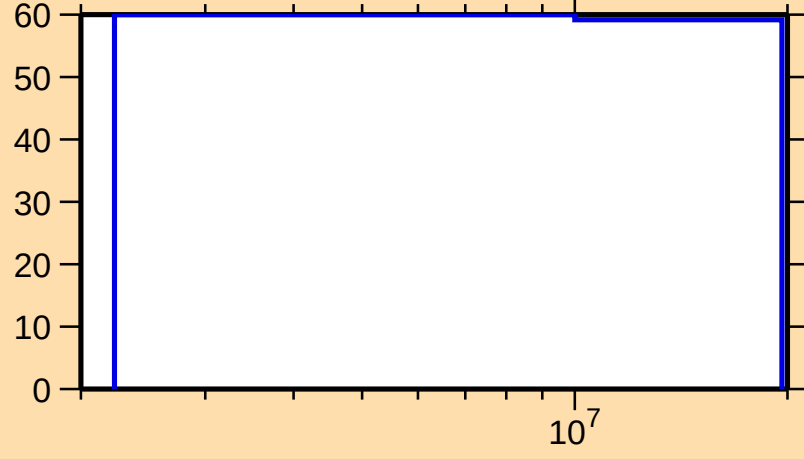
\Delta\sigma/\sigma vs. E for ^{101}\text{Cd}(n,n\text{cont.})
