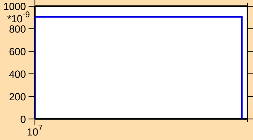
\sigma vs. E for ^{101}\text{Cd}(n,\text{pt})
