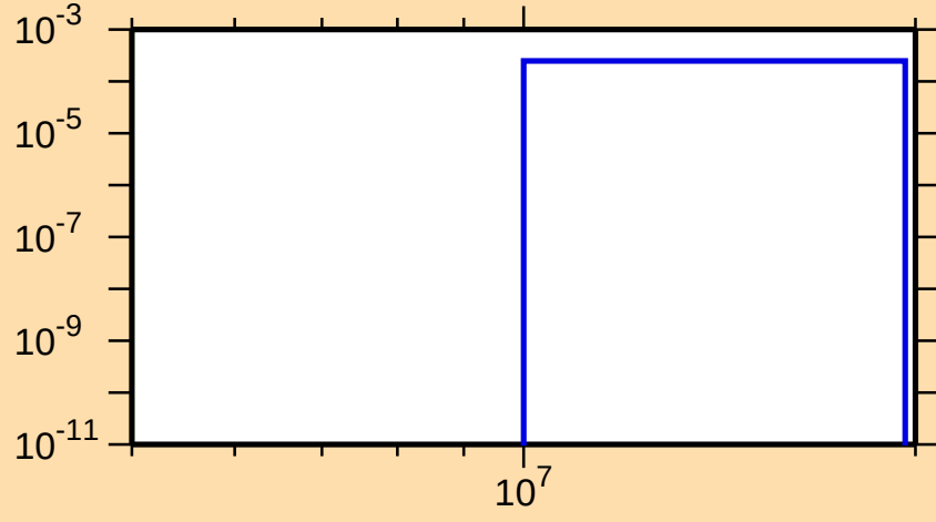
\sigma vs. E for ^{101}\text{Cd}(n,\text{pd})
