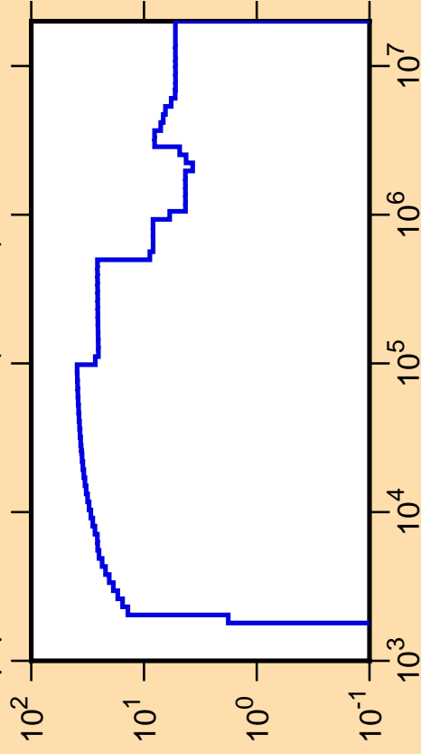
\Delta\mu/\mu vs. E for ^{102}\text{Cd}(\text{mt251})
