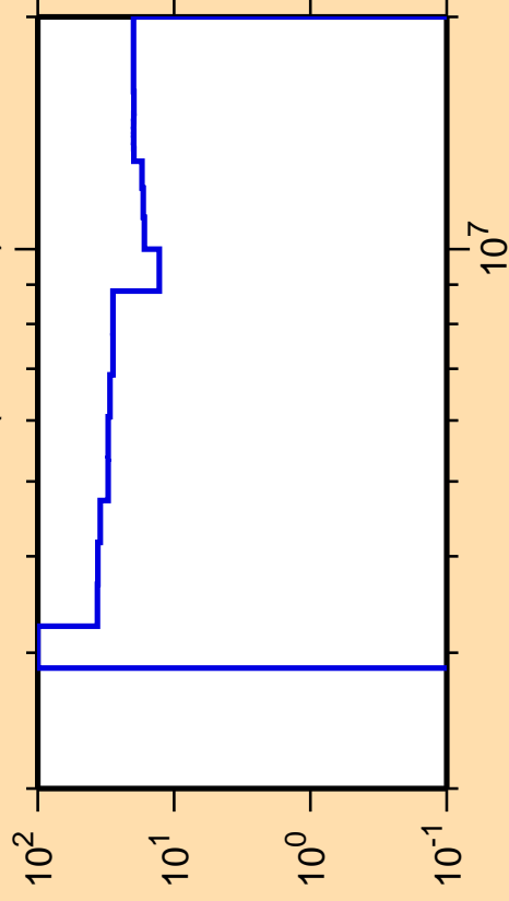
\Delta\sigma/\sigma vs. E for ^{102}\text{Cd}(n,\text{ncont.})
