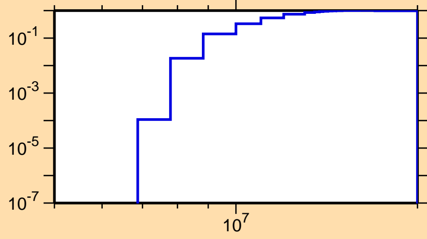
\sigma vs. E for ^{102}\text{Cd}(n,np)
