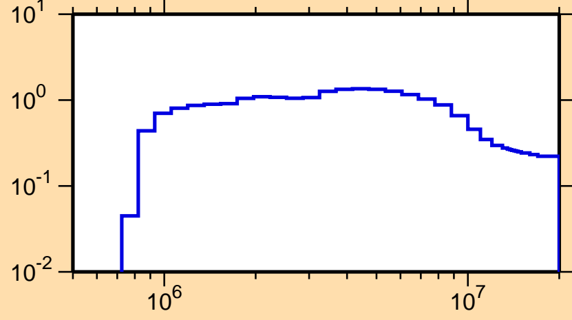
\sigma vs. E for ^{102}\text{Cd}(n,\text{inel.})
