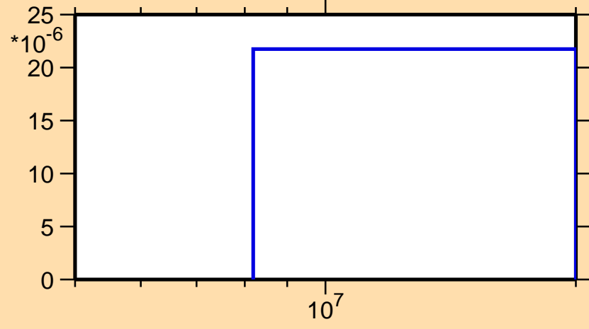
\sigma vs. E for ^{102}\text{Cd}(n,\text{pd})
