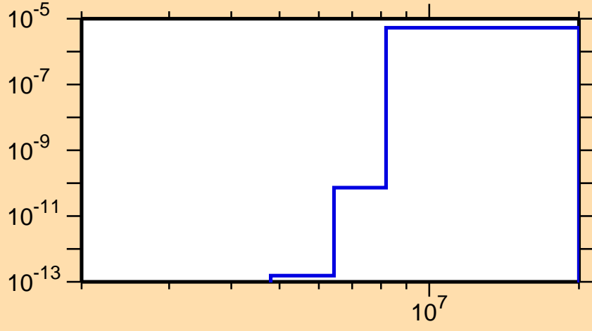
\sigma vs. E for ^{102}\text{Cd}(n,\text{He3})
