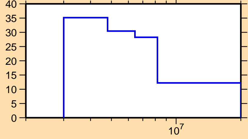
\Delta\sigma/\sigma vs. E for ^{102}\text{Cd}(n,ncont.)
