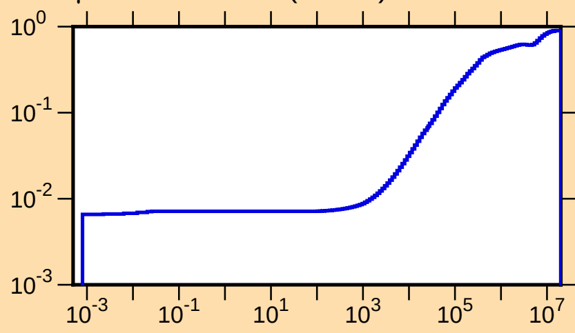
\mu vs. E for ^{103}\text{Cd}(\text{mt251})
