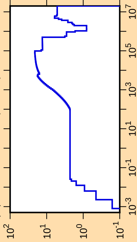
\Delta\mu/\mu vs. E for ^{103}\text{Cd}(\text{mt251})
