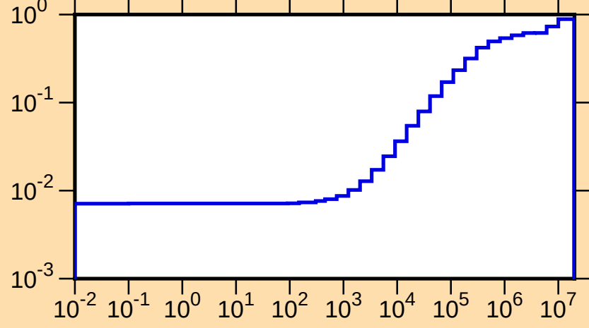
\mu vs. E for ^{103}\text{Cd}(\text{mt251})
