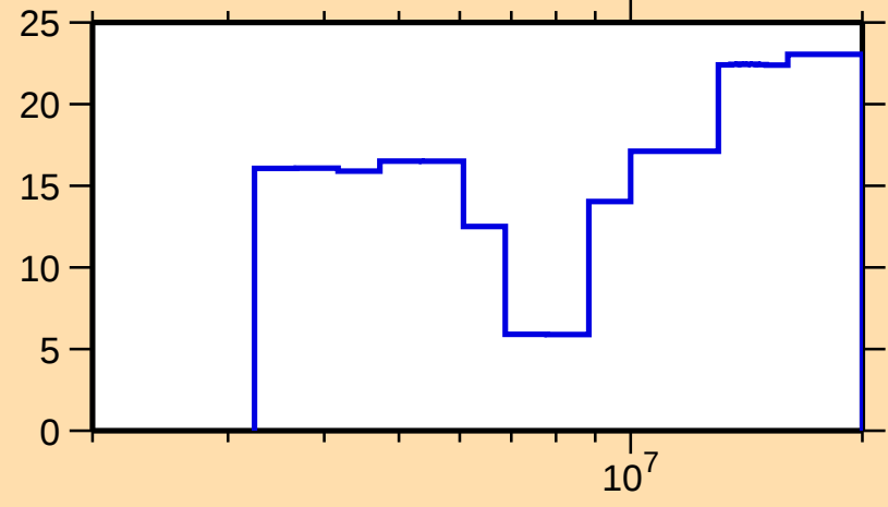
\Delta\sigma/\sigma vs. E for ^{104}\text{Cd}(\text{n},\text{el.})
