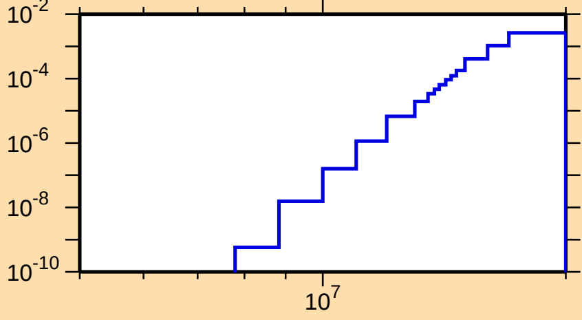
\sigma vs. E for ^{104}\text{Cd}(n,p\alpha)
