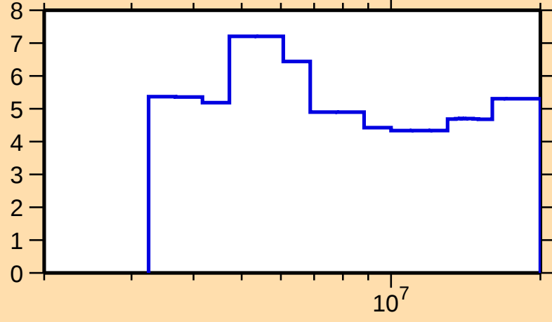
\Delta\sigma/\sigma vs. E for ^{104}\text{Cd}(\text{n},\text{nonel.})
