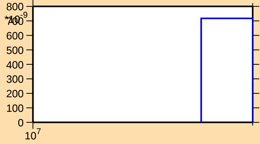
\sigma vs. E for ^{104}\text{Cd}(n,2np)
