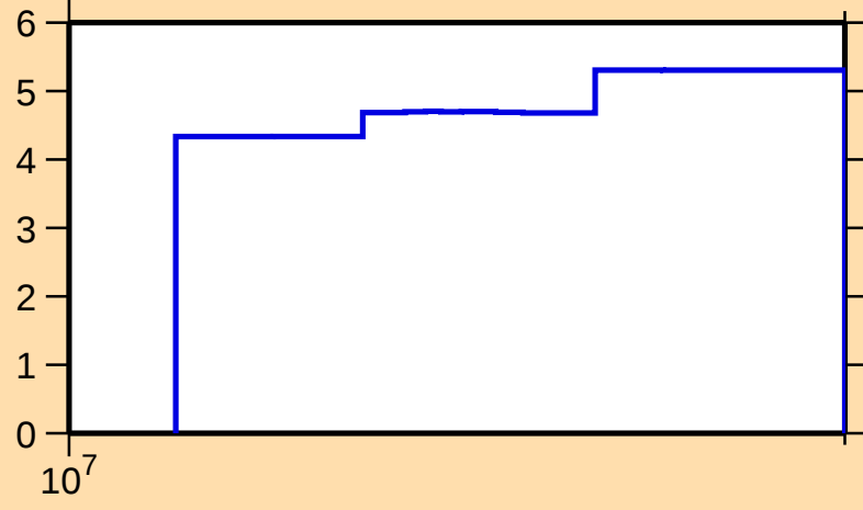
\Delta\sigma/\sigma vs. E for ^{104}\text{Cd}(n,\text{nonel.})
