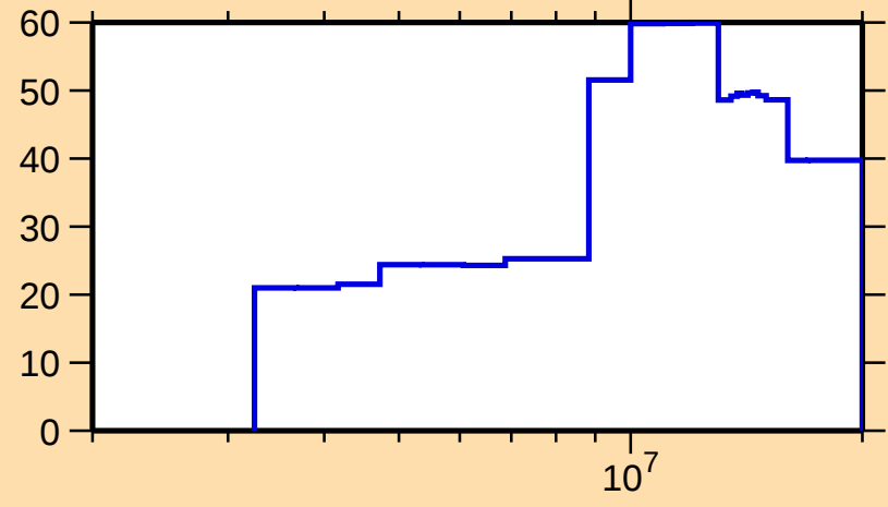
\Delta\sigma/\sigma vs. E for ^{104}\text{Cd}(\text{n},\text{inel.})
