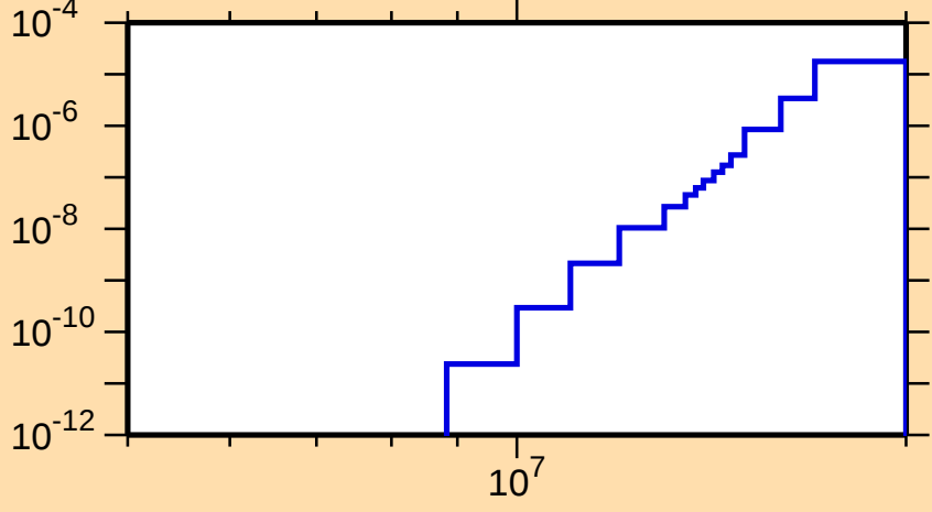
\sigma vs. E for ^{104}\text{Cd}(n,\text{He}3)
