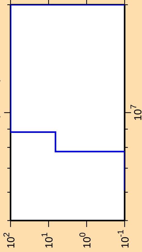
\Delta\sigma/\sigma vs. E for ^{104}\text{Cd}(n,\text{He}3)
