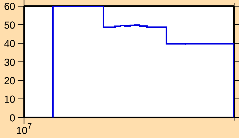
\Delta\sigma/\sigma vs. E for ^{104}\text{Cd}(n,\text{inel.})
