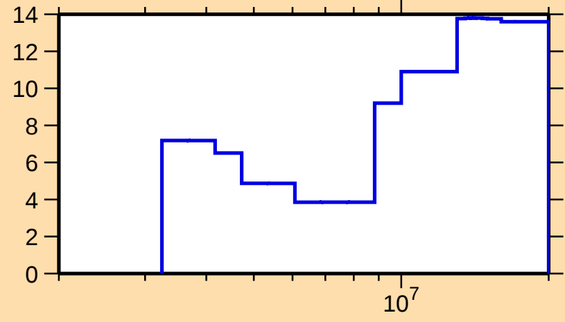
\Delta\sigma/\sigma vs. E for ^{104}\text{Cd}(\text{n},\text{tot.})
