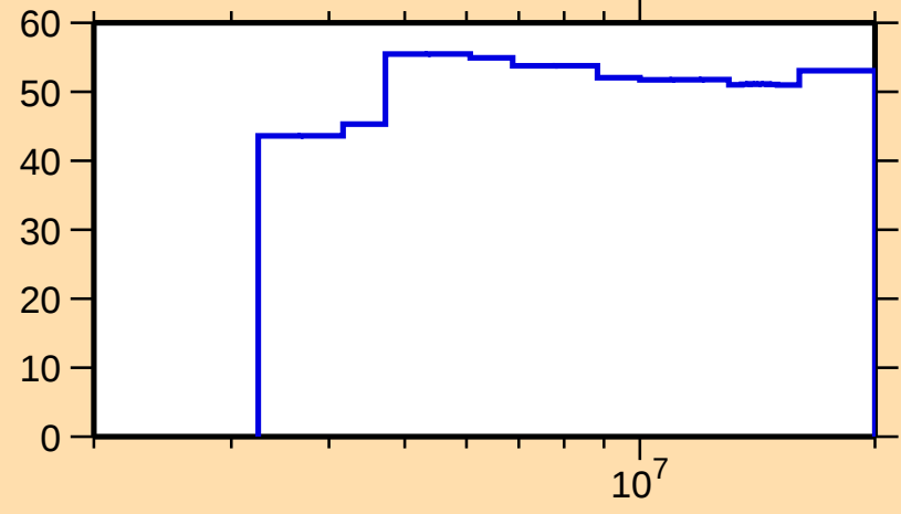
\Delta\sigma/\sigma vs. E for ^{104}\text{Cd}(n,n_1)
