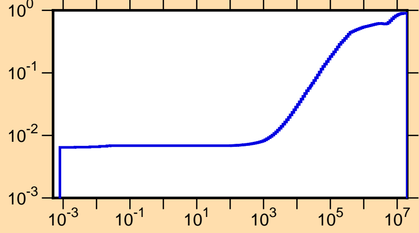
\mu vs. E for ^{105}\text{Cd}(\text{mt251})
