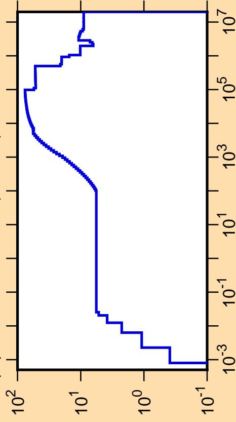
\Delta\mu/\mu vs. E for ^{105}\text{Cd}(\text{mt251})
