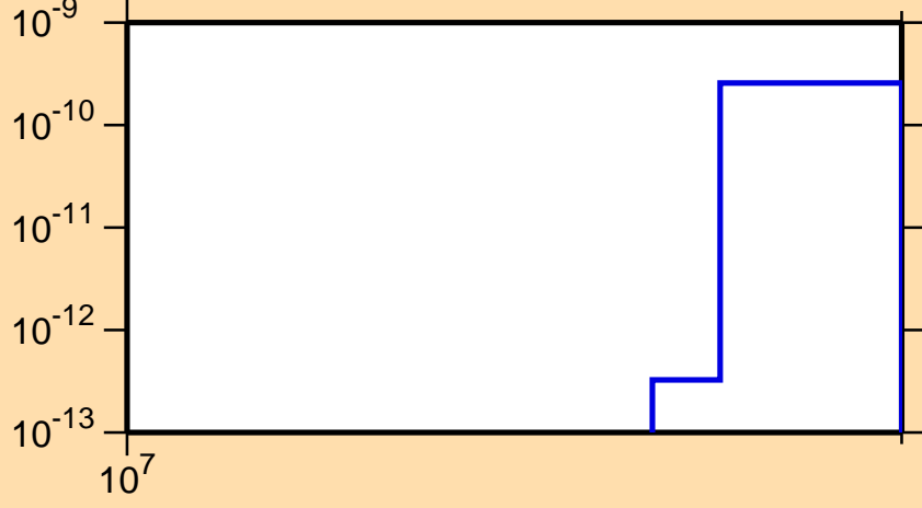
\sigma vs. E for ^{105}\text{Cd} (mt 34)
