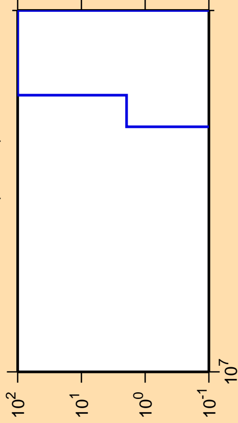
\Delta\sigma/\sigma vs. E for ^{105}\text{Cd} (mt 34)
