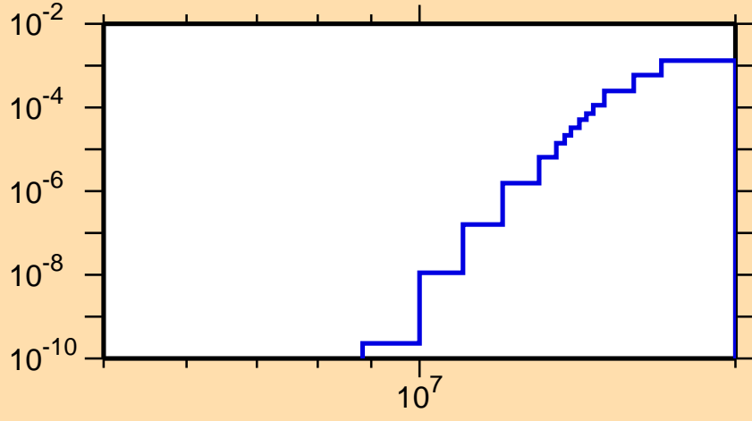
\sigma vs. E for ^{105}\text{Cd}(n,t)
