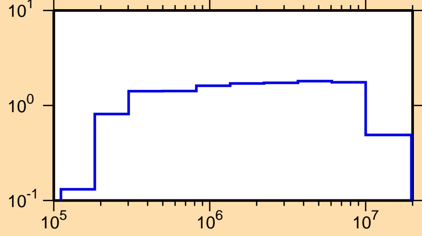
\sigma vs. E for ^{105}\text{Cd}(n,\text{inel.})
