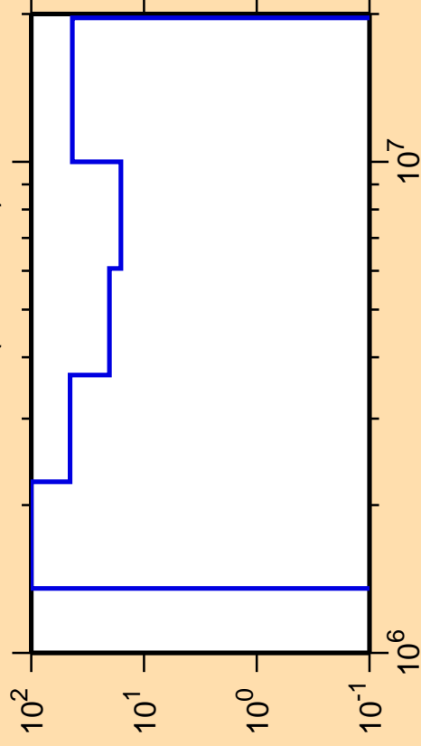
\Delta\sigma/\sigma vs. E for ^{105}\text{Cd}(n,\text{ncont.})
