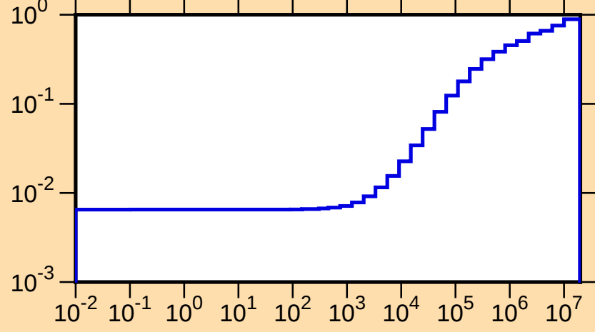
\mu vs. E for ^{106}\text{Cd}(\text{mt251})
