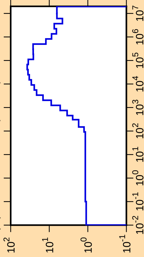
\Delta\mu/\mu vs. E for ^{106}\text{Cd}(\text{mt251})
