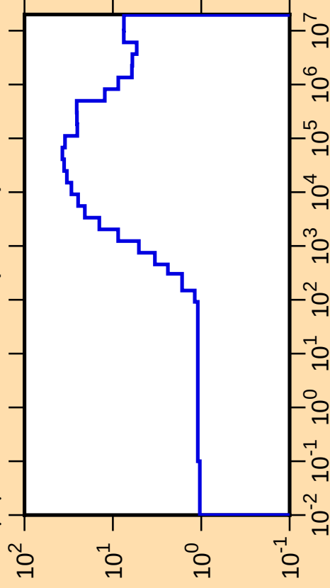
\Delta\mu/\mu vs. E for ^{108}\text{Cd}(\text{mt251})
