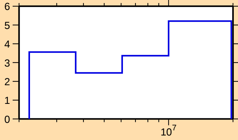
\Delta\sigma/\sigma vs. E for ^{110}\text{Cd}(\text{n},\text{tot.})
