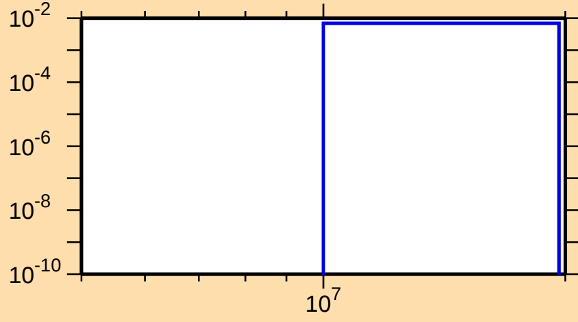
\sigma vs. E for ^{110}\text{Cd}(n,np)
