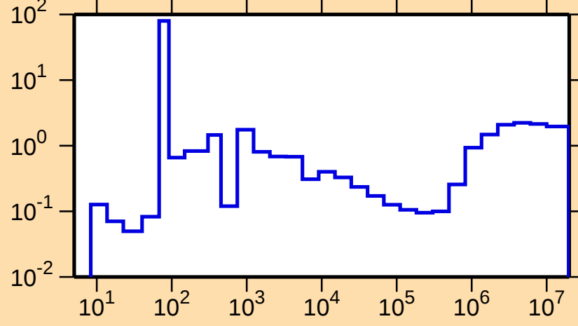
\sigma vs. E for ^{110}\text{Cd}(n,\text{nonel.})
