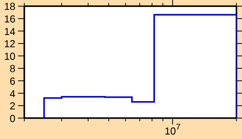
\Delta\sigma/\sigma vs. E for ^{110}\text{Cd}(\text{n},\text{inel.})
