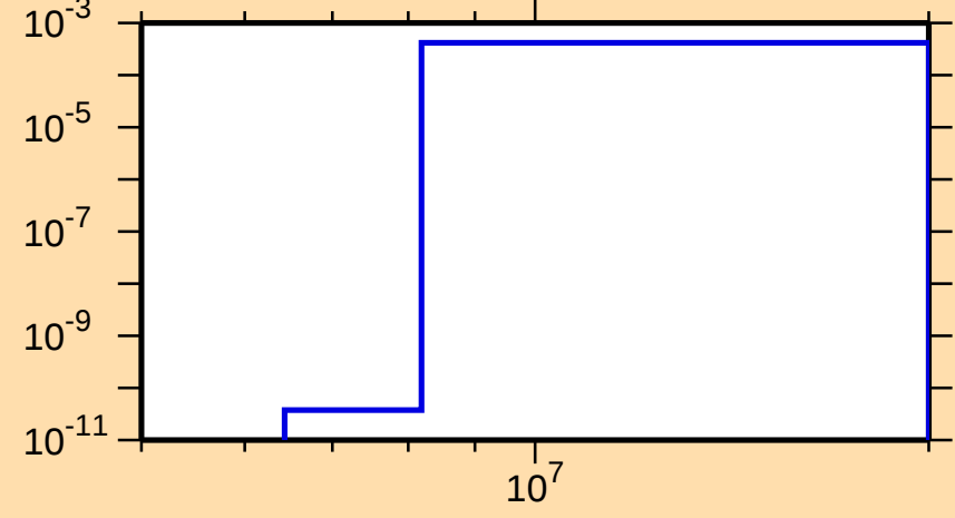
\sigma vs. E for ^{110}\text{Cd}(n,\alpha)
