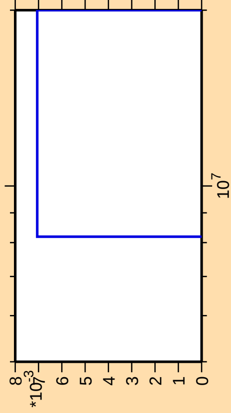
\Delta\sigma/\sigma vs. E for ^{110}\text{Cd}(n,\text{pd})
