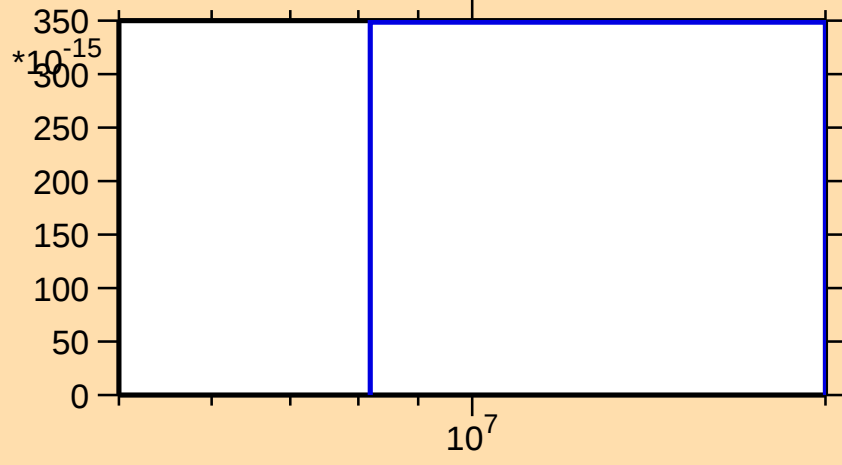
\sigma vs. E for ^{110}\text{Cd}(n,2np)
