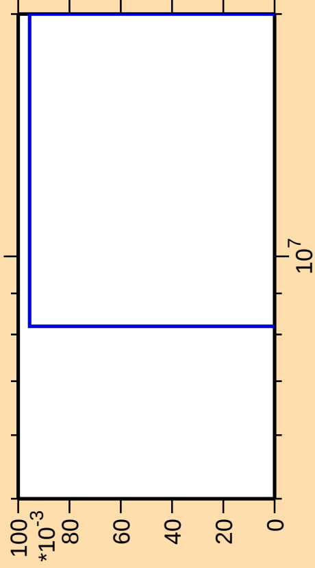
\Delta\sigma/\sigma vs. E for ^{110}\text{Cd}(n,\text{nt})
