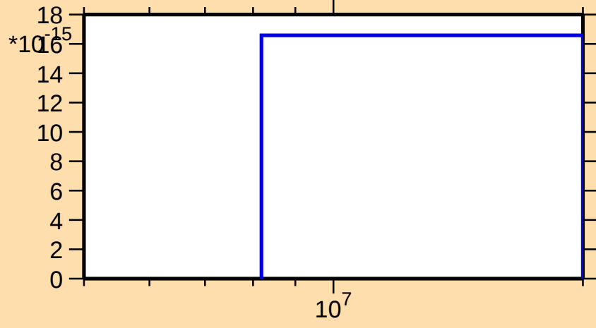
\sigma vs. E for ^{110}\text{Cd}(n,\text{nt})
