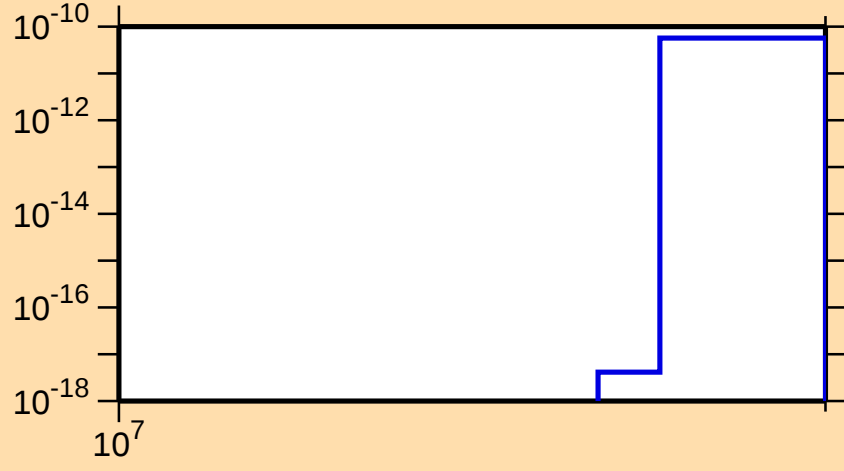
\sigma vs. E for ^{111}\text{Cd}(n,\text{nt})
