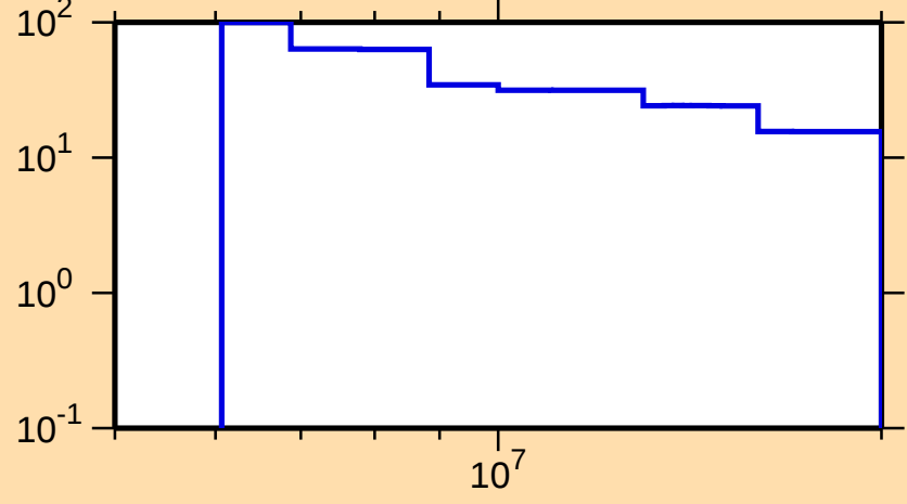
\Delta\sigma/\sigma vs. E for ^{111}\text{Cd}(n,2n)
