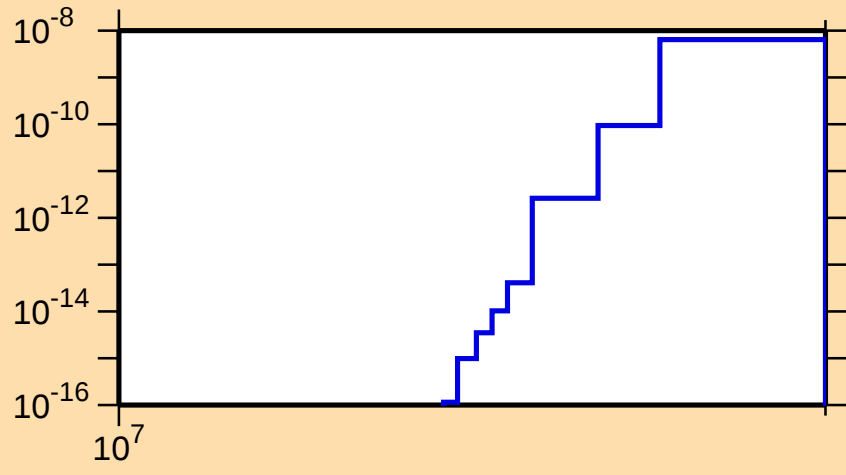
\sigma vs. E for ^{111}\text{Cd}(n,\text{He}3)
