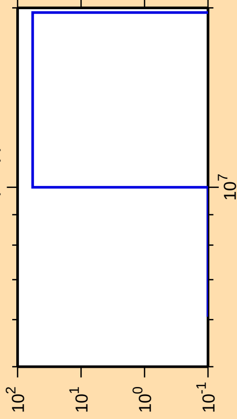
\Delta\sigma/\sigma vs. E for ^{111}\text{Cd}(n,np)
