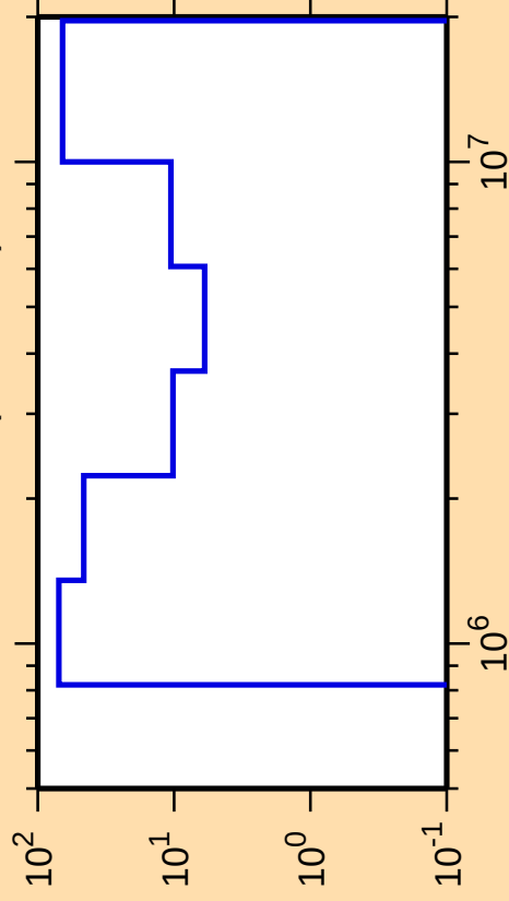
\Delta\sigma/\sigma vs. E for ^{111}\text{Cd}(\text{n},\text{ncont.})
