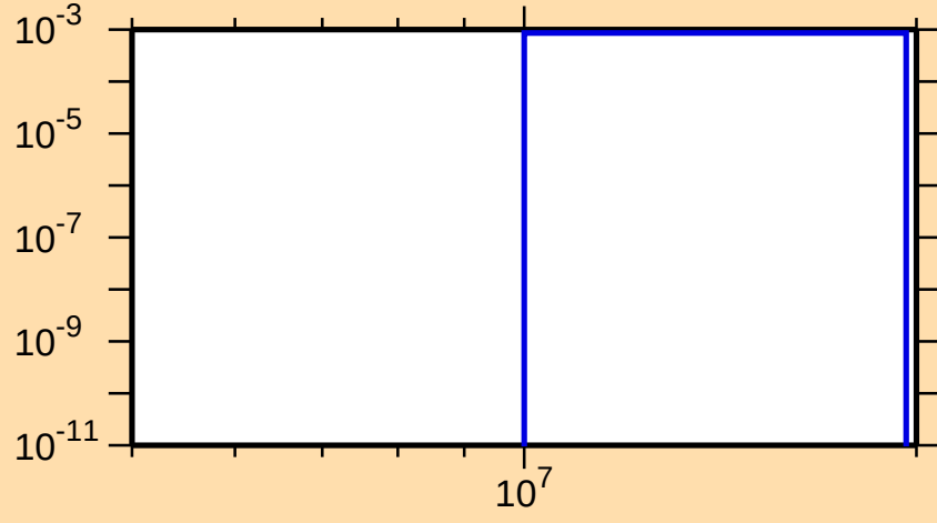
\sigma vs. E for ^{111}\text{Cd}(n,np)
