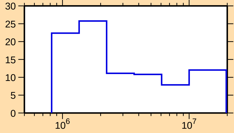
\Delta\sigma/\sigma vs. E for ^{111}\text{Cd}(\text{n},\text{el.})
