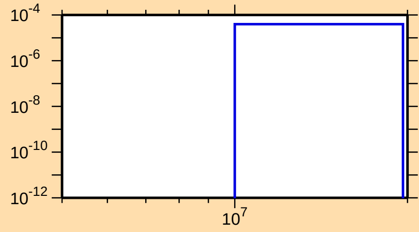
\sigma vs. E for ^{111}\text{Cd}(n,t)
