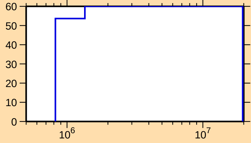
\Delta\sigma/\sigma vs. E for ^{111}\text{Cd}(n,n_1)
