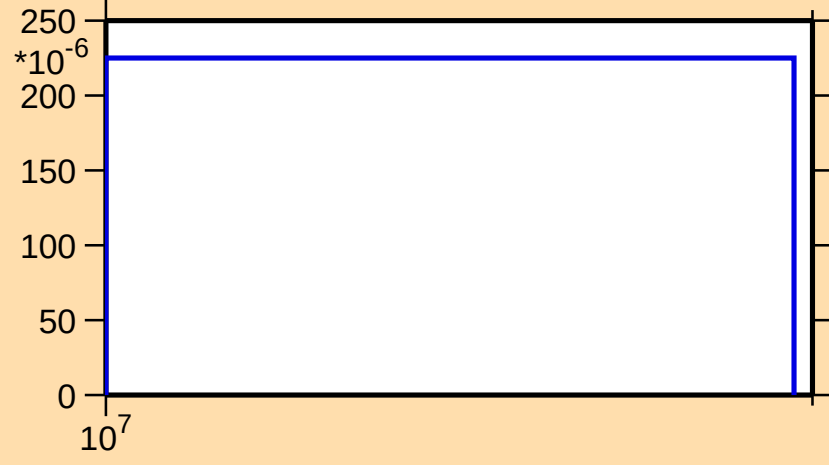
\sigma vs. E for ^{111}\text{Cd}(n,3n)
