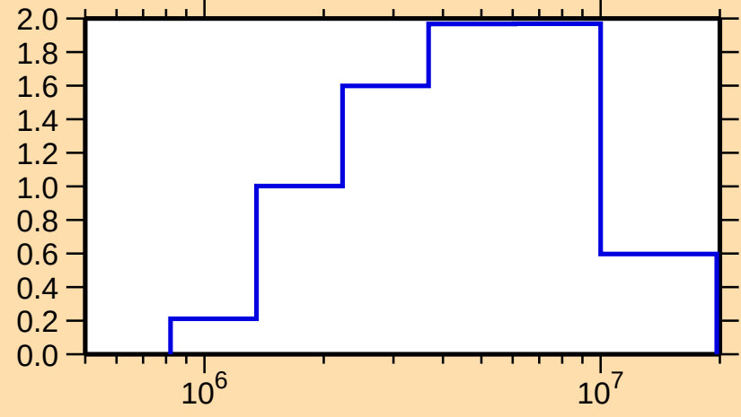
\sigma vs. E for ^{111}\text{Cd}(n,n\text{cont.})
