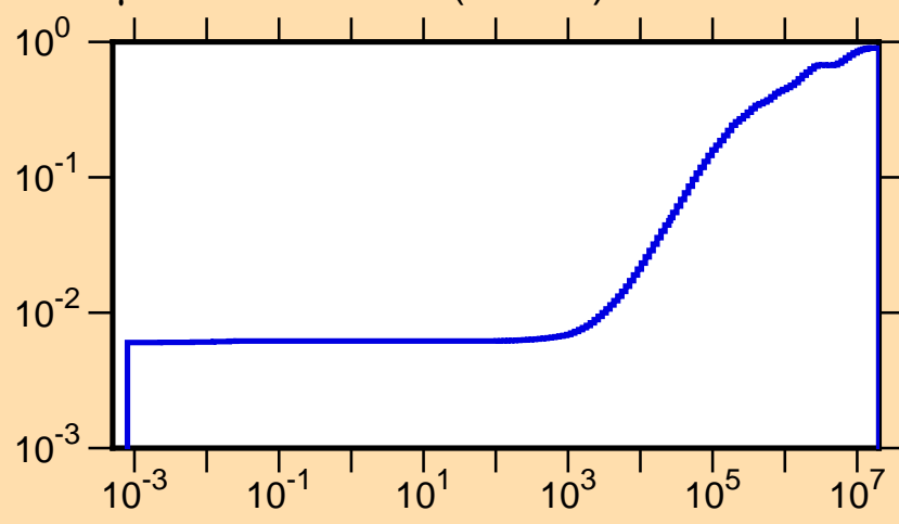
\mu vs. E for ^{112}\text{Cd}(\text{mt251})
