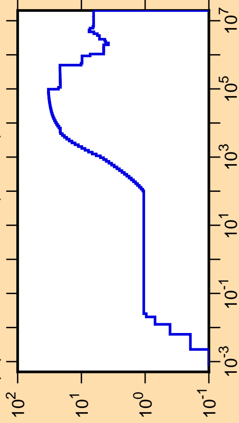
\Delta\mu/\mu vs. E for ^{112}\text{Cd}(\text{mt251})
