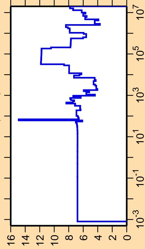
\Delta\sigma/\sigma vs. E for ^{112}\text{Cd}(n,\text{el.})
