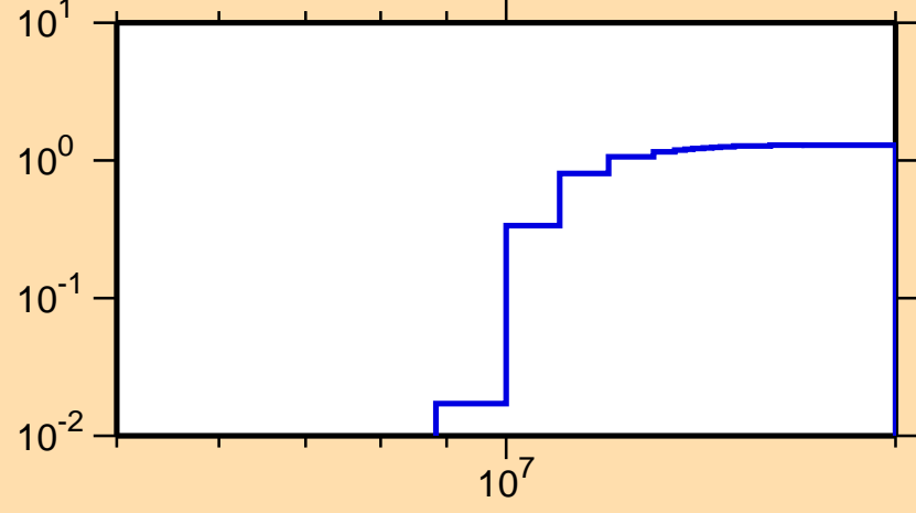
\sigma vs. E for ^{112}\text{Cd}(n,2n)
