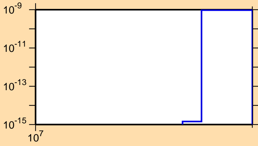
\sigma vs. E for ^{112}\text{Cd}(n,\text{nd})
