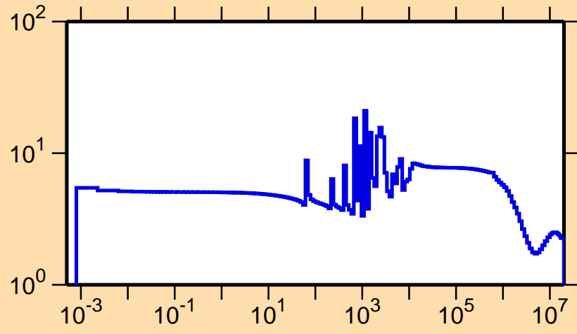
\sigma vs. E for ^{112}\text{Cd}(n,\text{el.})
