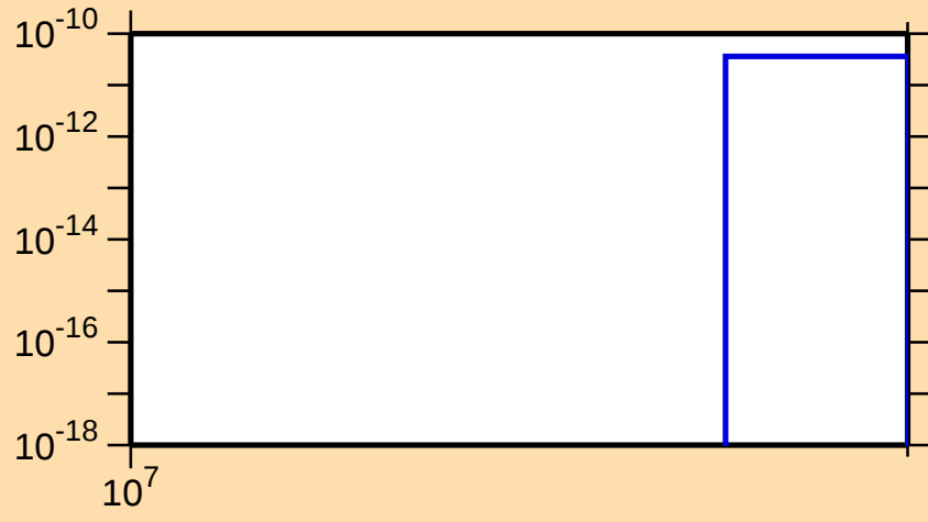
\sigma vs. E for ^{113}\text{Cd}(n,\text{nt})
