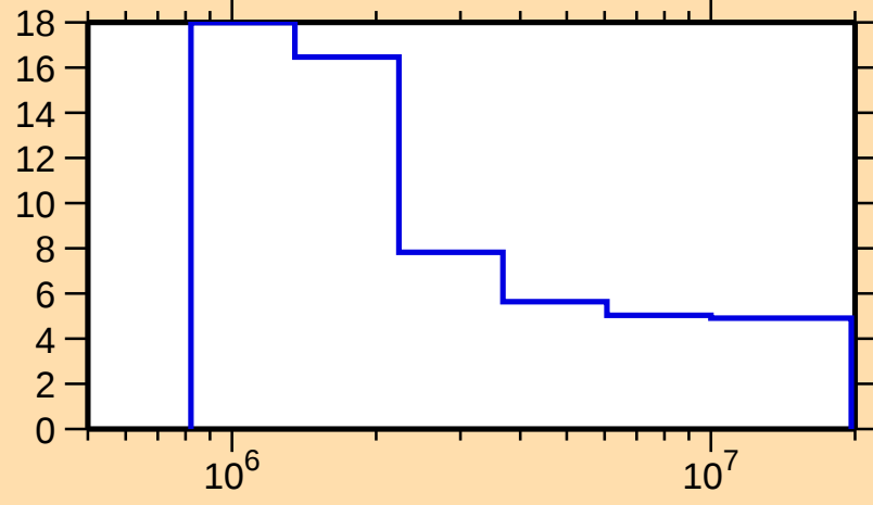
\Delta\sigma/\sigma vs. E for ^{113}\text{Cd}(\text{n},\text{nonel.})
