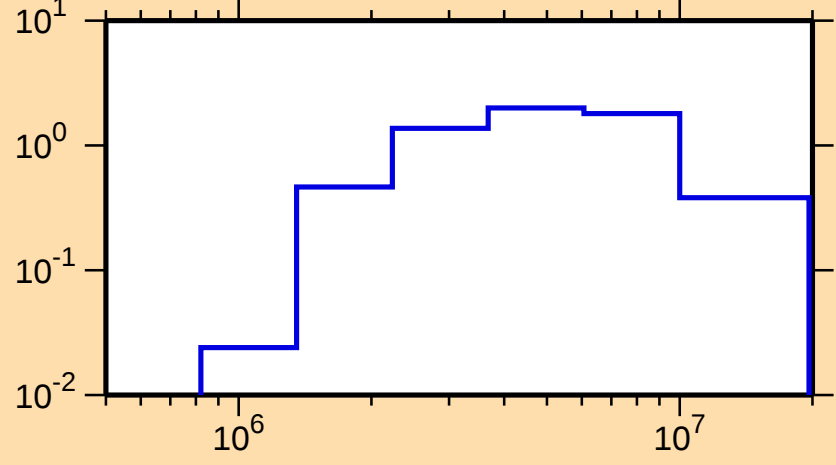
\sigma vs. E for ^{113}\text{Cd}(n,n\text{cont.})
