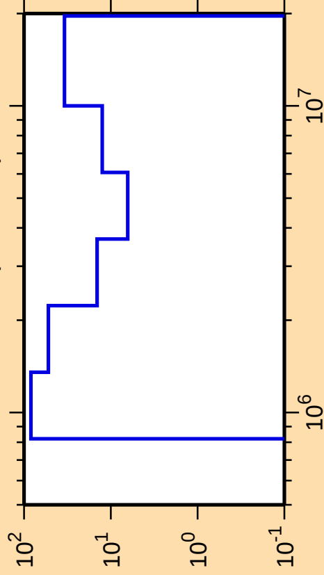
\Delta\sigma/\sigma vs. E for ^{113}\text{Cd}(\text{n},\text{ncont.})
