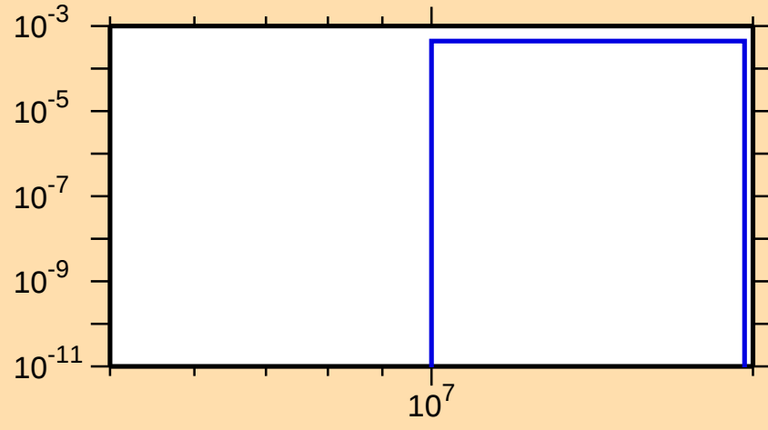
\sigma vs. E for ^{113}\text{Cd}(n,d)
