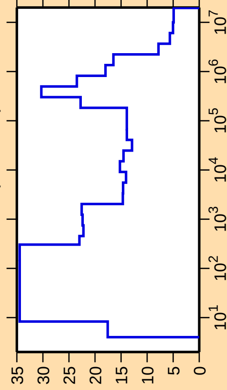
\Delta\sigma/\sigma vs. E for ^{113}\text{Cd}(n,\text{nonel.})
