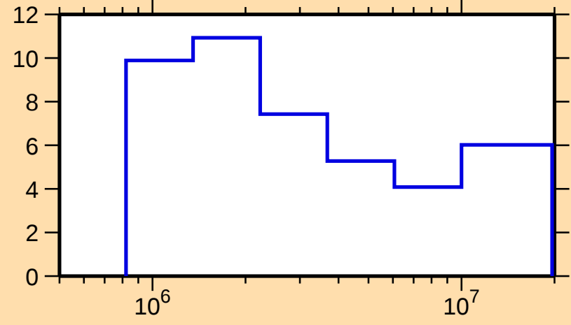
\Delta\sigma/\sigma vs. E for ^{113}\text{Cd}(\text{n},\text{tot.})
