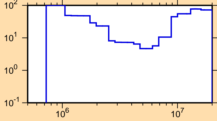
\Delta\sigma/\sigma vs. E for ^{113}\text{Cd}(n,n\text{cont.})
