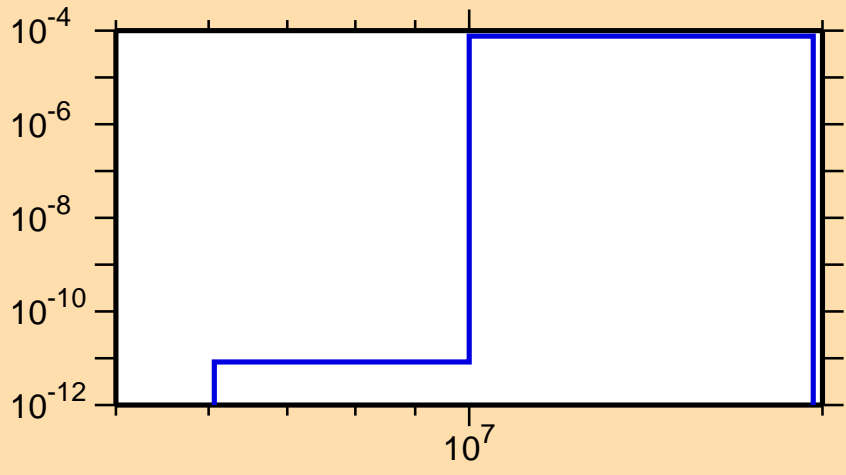
\sigma vs. E for ^{113}\text{Cd}(n,\alpha)
