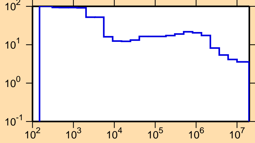
\Delta\sigma/\sigma vs. E for ^{113}\text{Cd}(n,\text{nonel.})
