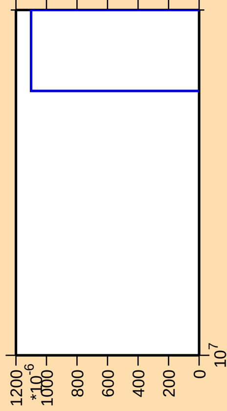
\Delta\sigma/\sigma vs. E for ^{114}\text{Cd}(n,2np)
