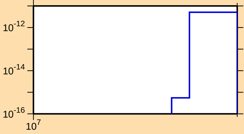
\sigma vs. E for ^{114}\text{Cd}(n,\text{He}3)
