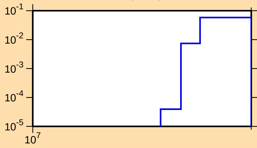
\sigma vs. E for ^{114}\text{Cd}(n,3n)
