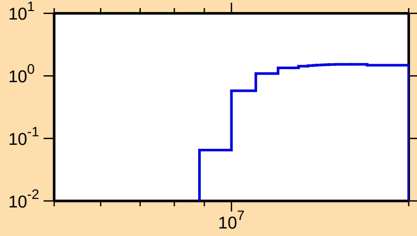
\sigma vs. E for ^{114}\text{Cd}(n,2n)
