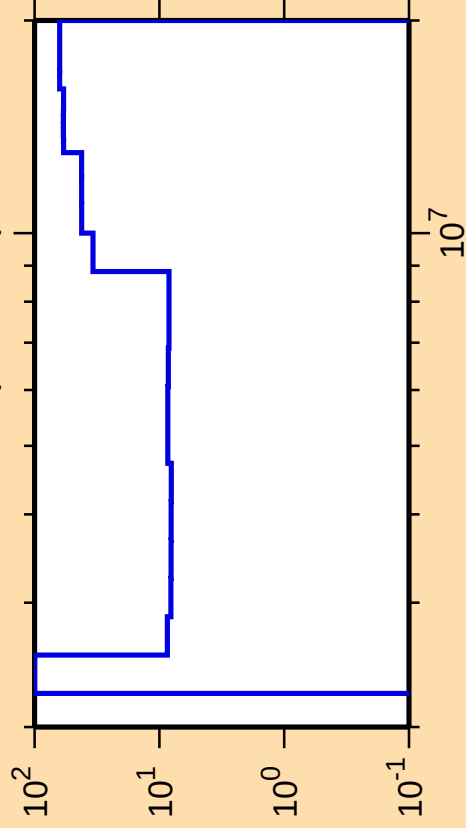
\Delta\sigma/\sigma vs. E for ^{114}\text{Cd}(\text{n,ncont.})
