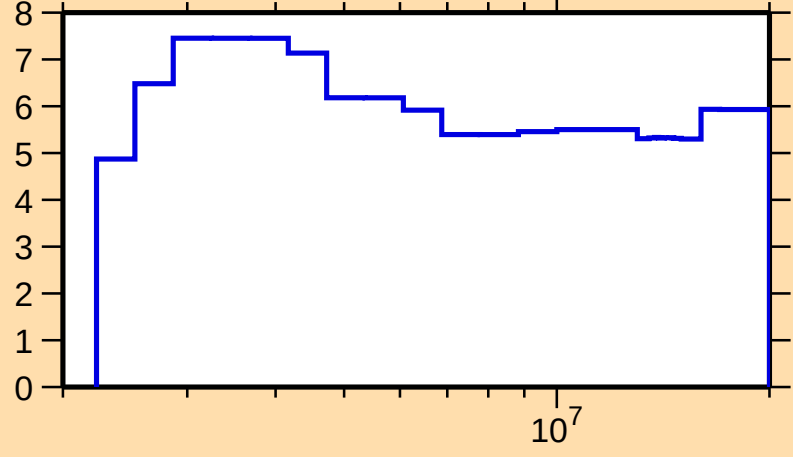
\Delta\sigma/\sigma vs. E for ^{114}\text{Cd}(\text{n},\text{nonel.})
