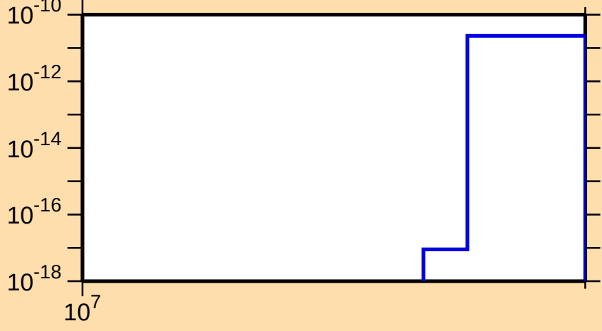
\sigma vs. E for ^{114}\text{Cd}(n,2n\alpha)
