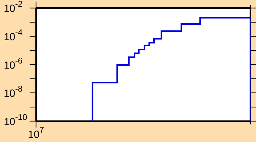
\sigma vs. E for ^{114}\text{Cd}(n,np)
