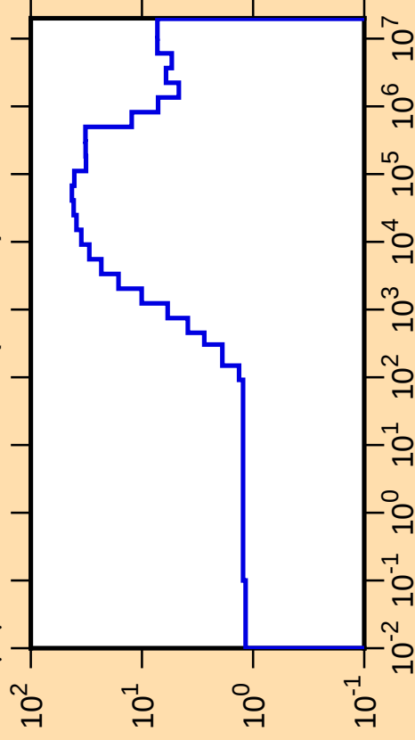
\Delta\mu/\mu vs. E for ^{114}\text{Cd}(\text{mt251})
