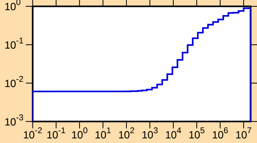
\mu vs. E for ^{114}\text{Cd}(\text{mt251})
