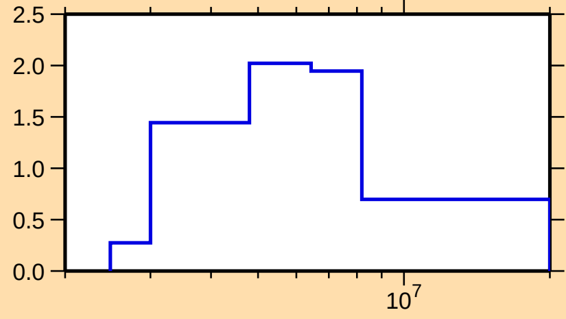
\sigma vs. E for ^{114}\text{Cd}(n,n\text{cont.})
