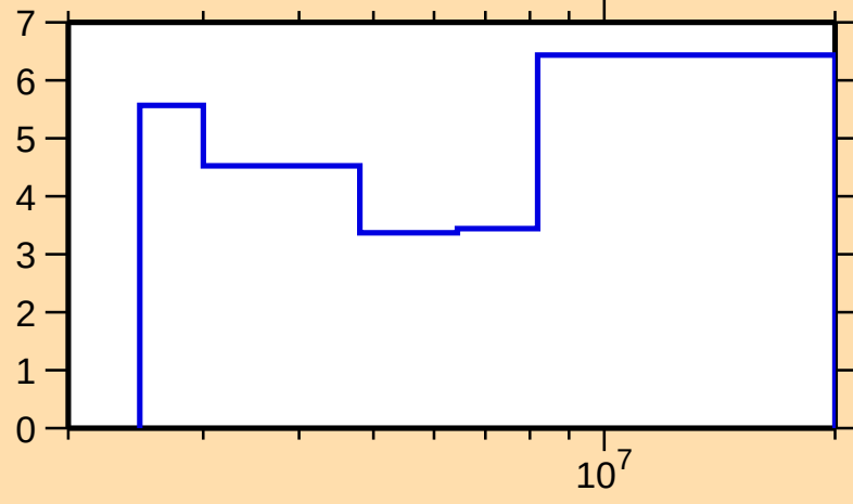
\Delta\sigma/\sigma vs. E for ^{114}\text{Cd}(\text{n},\text{tot.})
