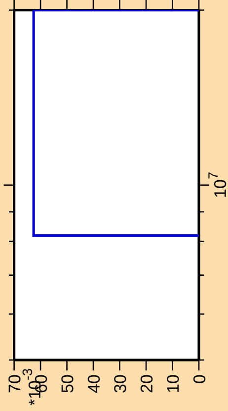
\Delta\sigma/\sigma vs. E for ^{114}\text{Cd}(n,\text{nt})
