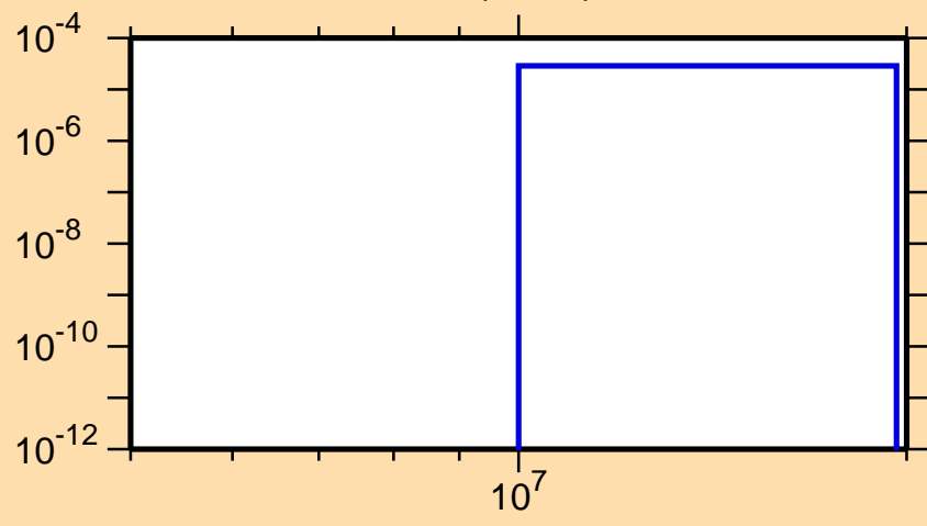
\sigma vs. E for ^{115}\text{Cd}(n,\alpha)
