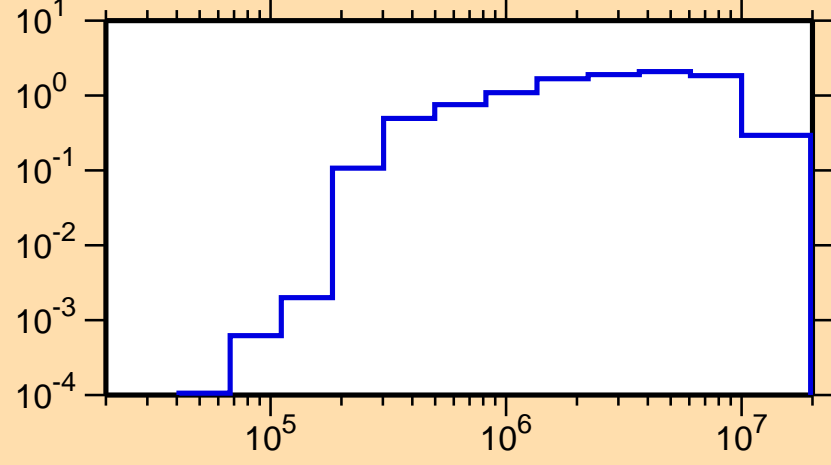
\sigma vs. E for ^{115}\text{Cd}(n,\text{inel.})
