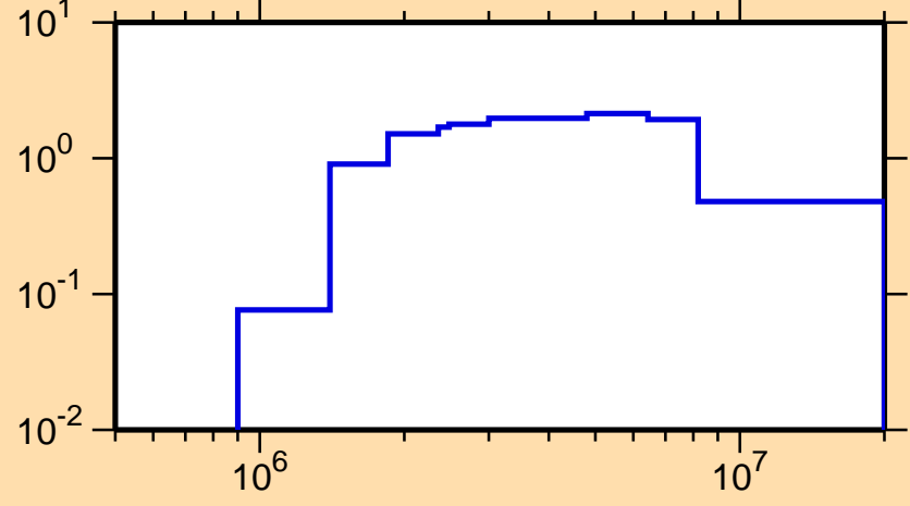
\sigma vs. E for ^{115}\text{Cd}(n,n\text{cont.})
