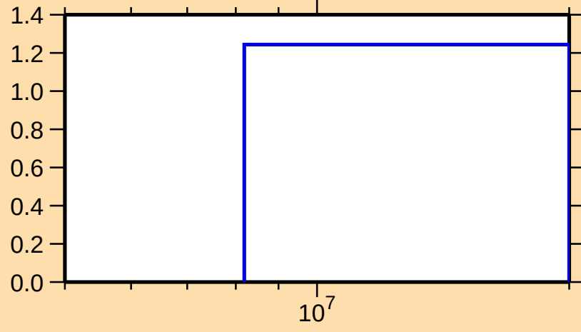
\sigma vs. E for ^{116}\text{Cd}(n,2n)
