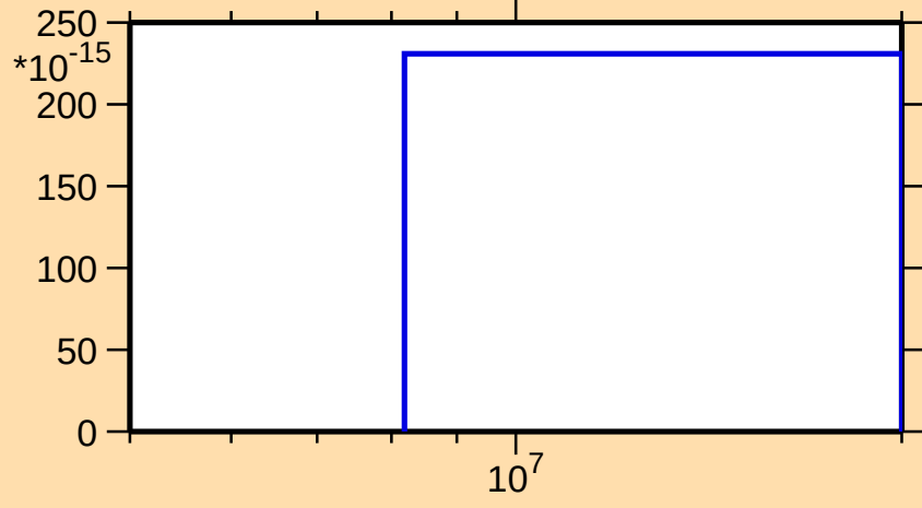
\sigma vs. E for ^{116}\text{Cd}(\text{n},\text{nd})
