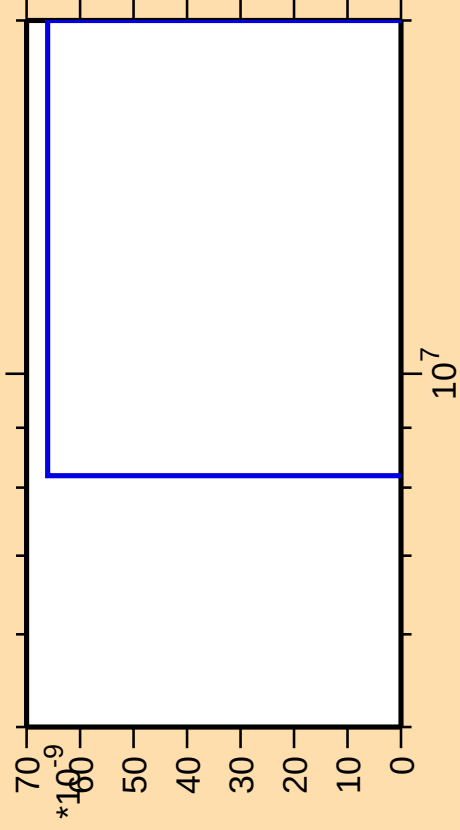
\Delta\sigma/\sigma vs. E for ^{116}\text{Cd}(n,2np)
