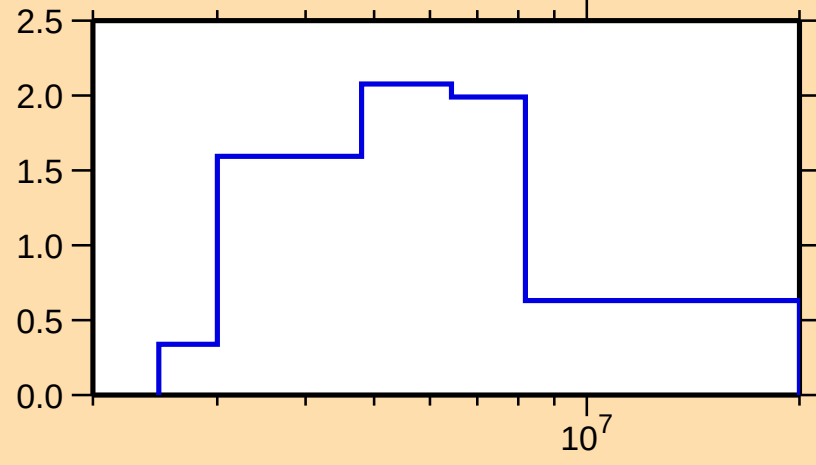
\sigma vs. E for ^{116}\text{Cd}(n,n\text{cont.})
