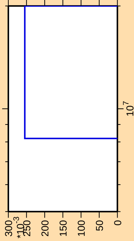
\Delta\sigma/\sigma vs. E for ^{116}\text{Cd}(n,\text{nt})
