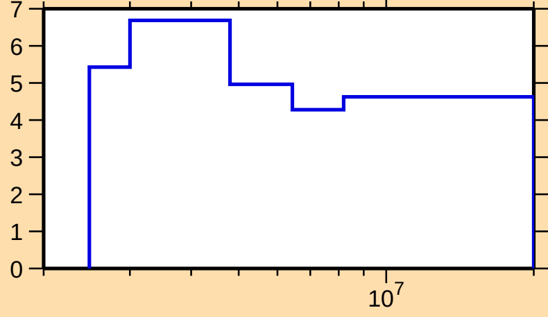
\Delta\sigma/\sigma vs. E for ^{116}\text{Cd}(\text{n},\text{nonel.})
