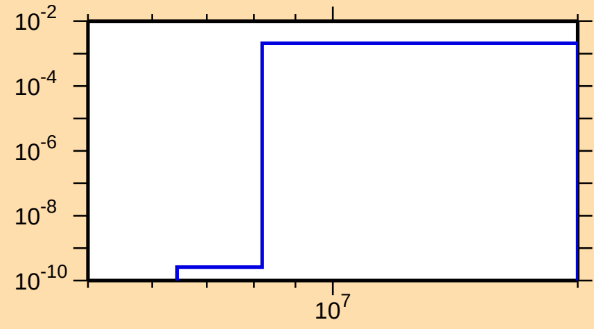
\sigma vs. E for ^{116}\text{Cd}(n,p)
