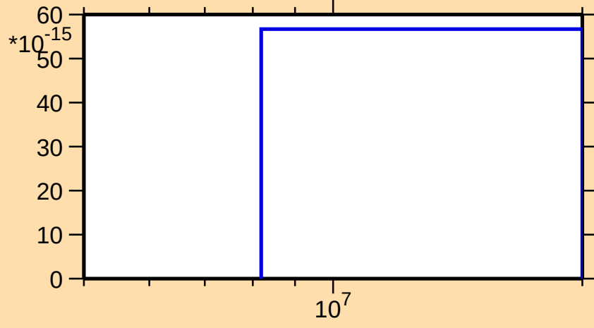
\sigma vs. E for ^{116}\text{Cd}(n,\text{nt})
