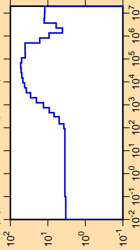
\Delta\mu/\mu vs. E for ^{117}\text{Cd}(\text{mt251})
