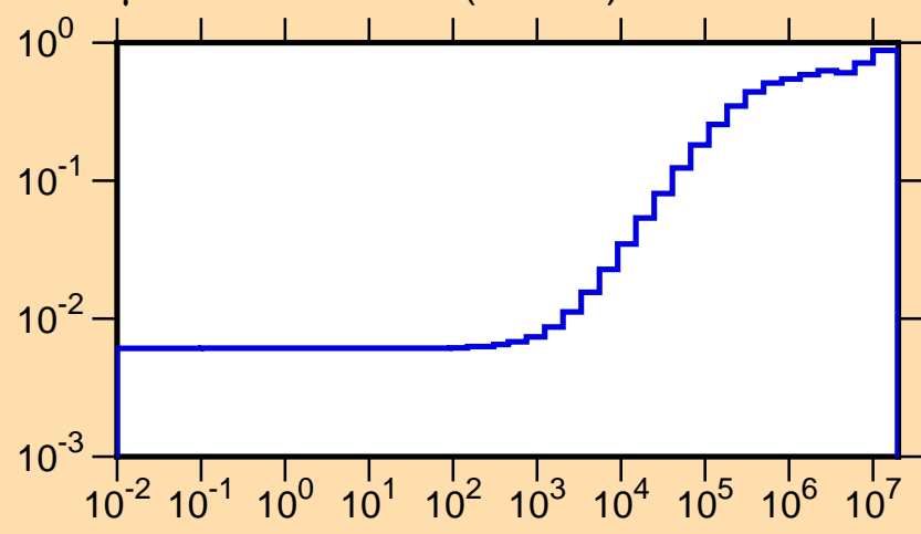
\mu vs. E for ^{117}\text{Cd}(\text{mt251})
