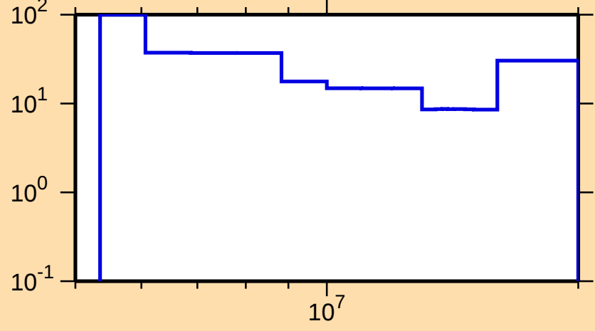
\Delta\sigma/\sigma vs. E for ^{117}\text{Cd}(n,2n)
