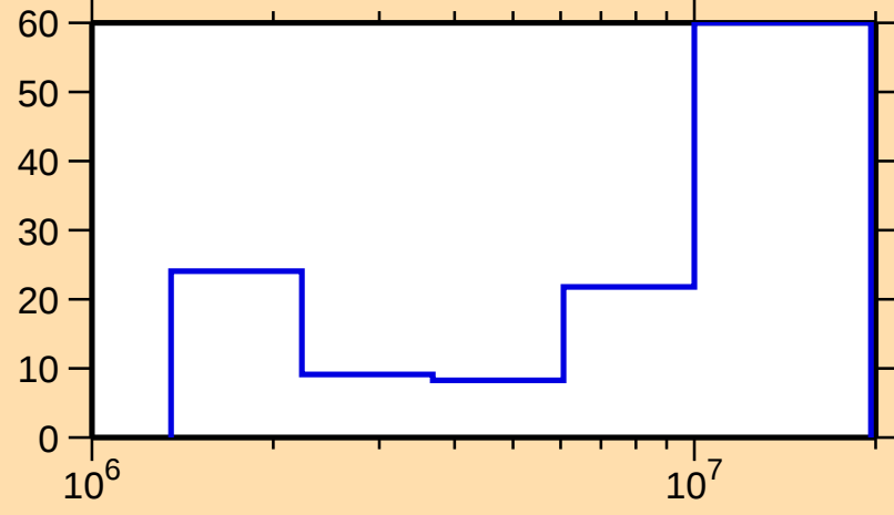
\Delta\sigma/\sigma vs. E for ^{117}\text{Cd}(n,n\text{cont.})
