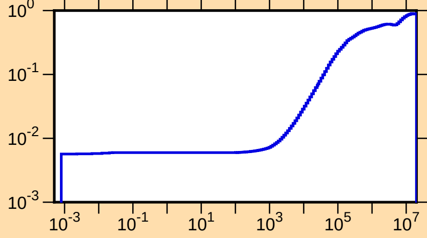
\mu vs. E for ^{119}\text{Cd}(\text{mt251})
