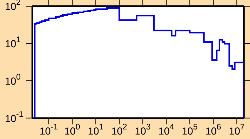
\Delta\sigma/\sigma vs. E for ^{119}\text{Cd}(n,\text{tot.})
