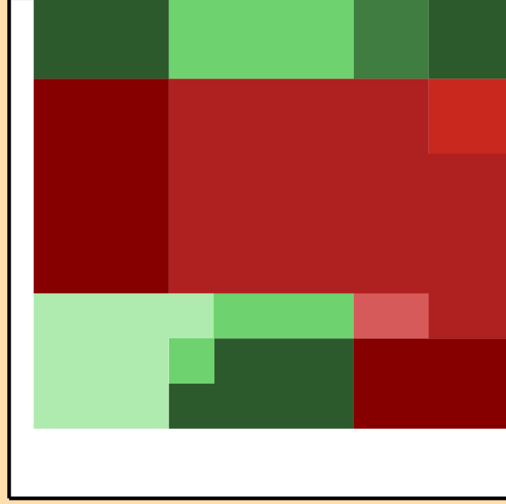
\Delta\sigma/\sigma vs. E for ^{121}\text{Cd}(n,p)
