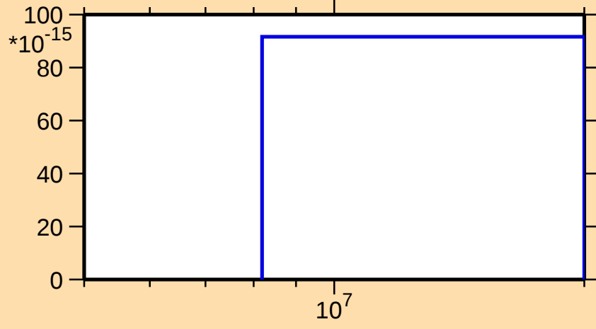
\sigma vs. E for ^{121}\text{Cd}(n,\text{nt})
