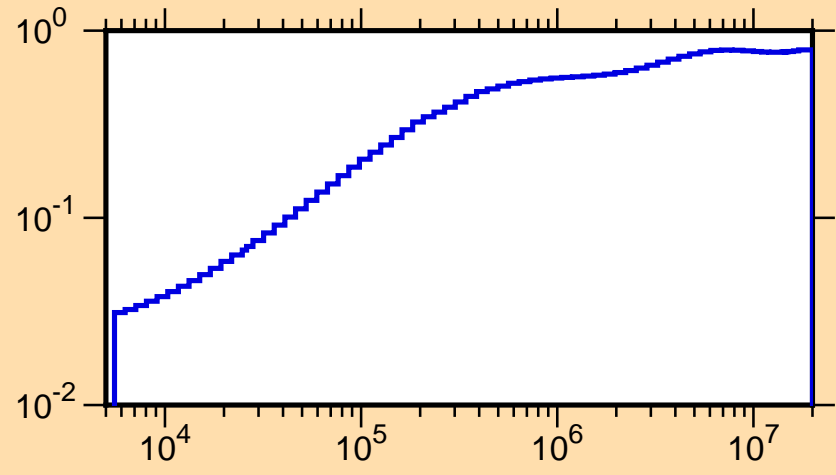
\mu vs. E for ^{33}\text{Cl}(\text{mt251})
