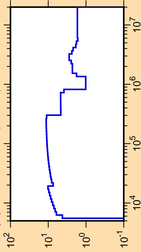
\Delta\mu/\mu vs. E for ^{33}\text{Cl}(\text{mt251})
