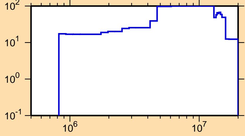
\Delta\sigma/\sigma vs. E for ^{33}\text{Cl}(n,\text{inel.})
