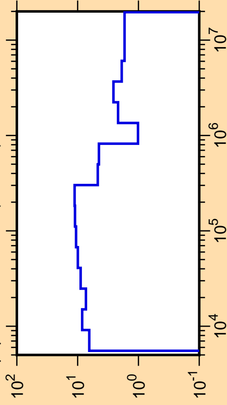
\mu vs. E for ^{33}\text{Cl}(\text{mt251})
